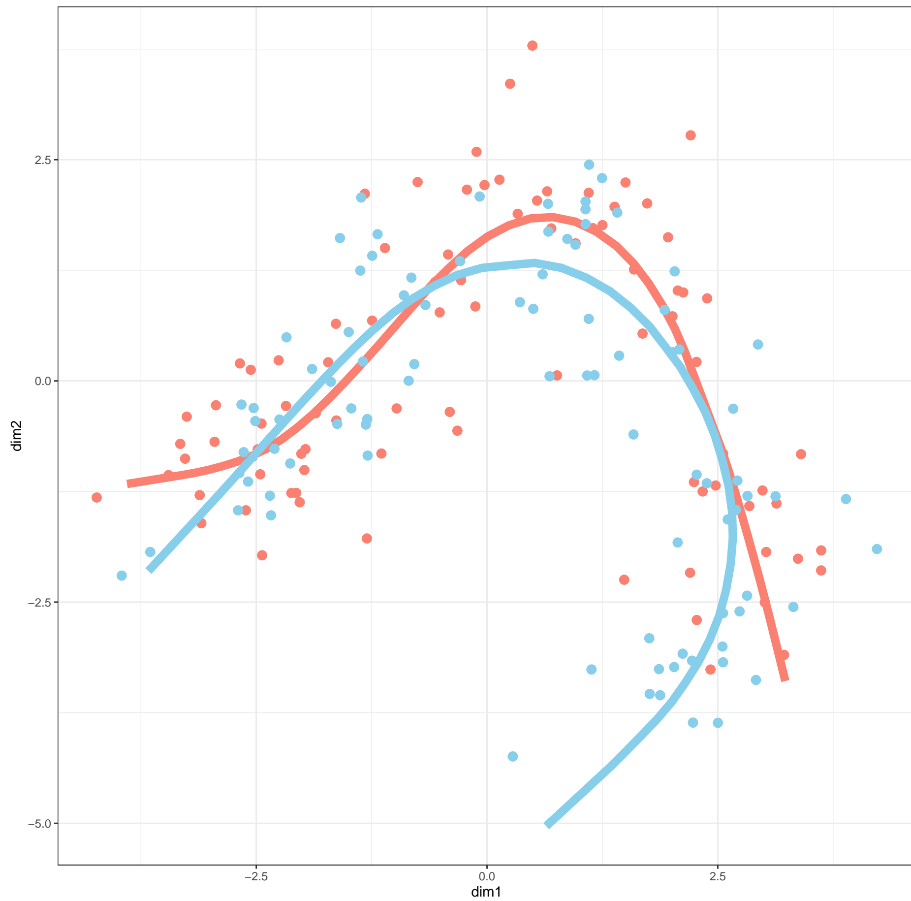
Y scaled to X * X basis -> curve
