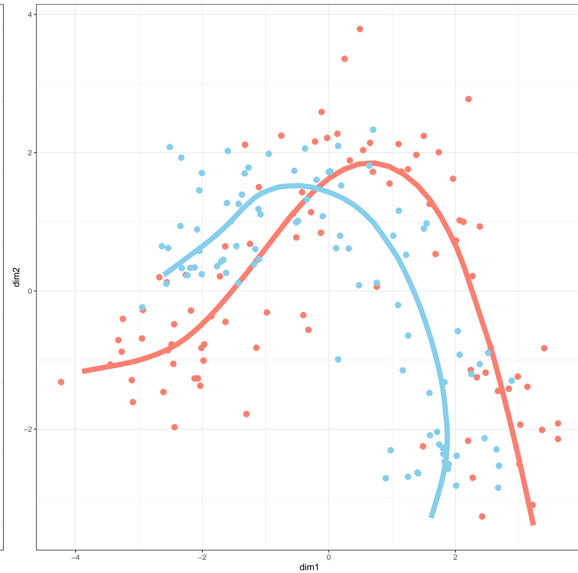
Y basis procrustes to X basis -> curve
