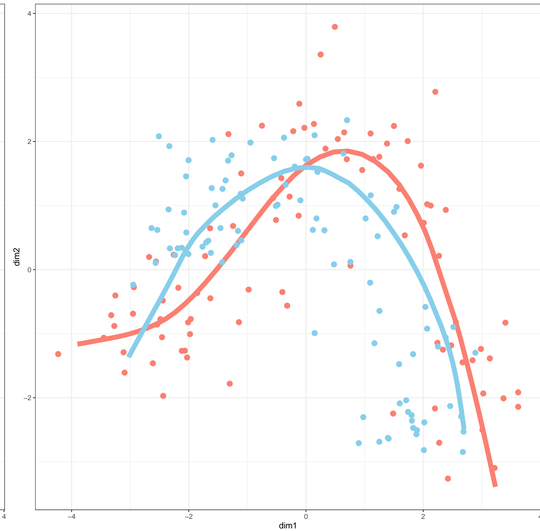
Y basis procrustes to X basis -> curve > Y curve procrustes to X curve
