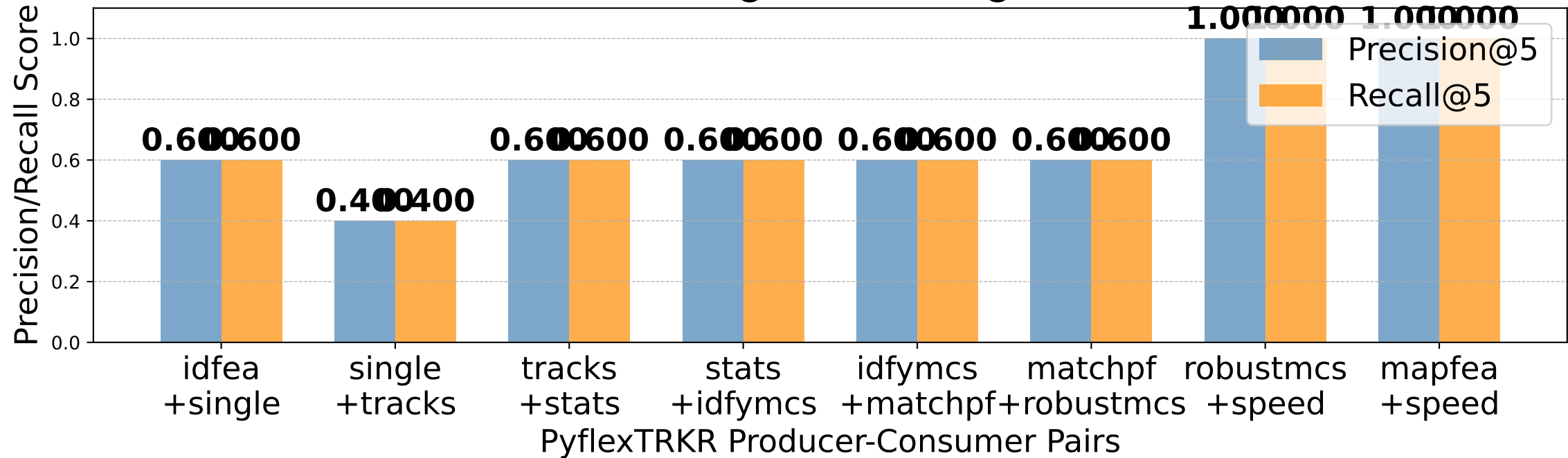
SPM Precision@5 and Recall@5 Metrics
