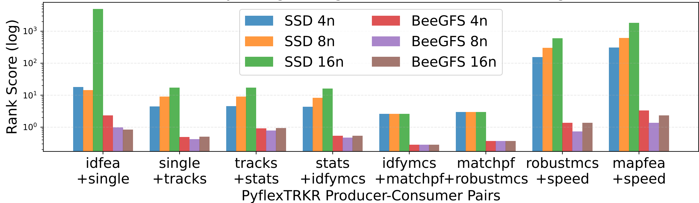
Rank Score by Storage Configuration (SSD and BeeGFS) - Log Scale
