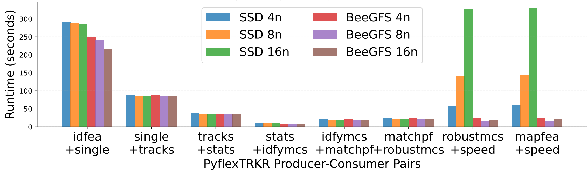
Workflow Time by Storage Configuration (SSD and BeeGFS)
