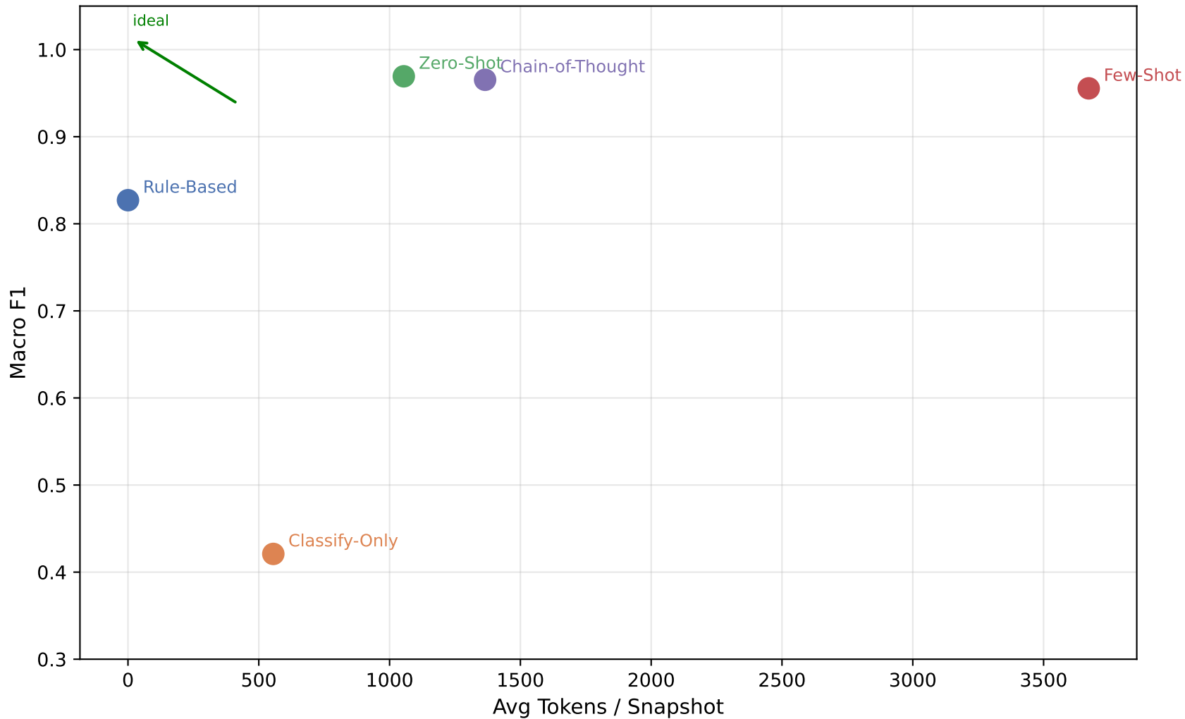
Cost vs. Accuracy Pareto (lower-left = cheaper, upper-left = better)
