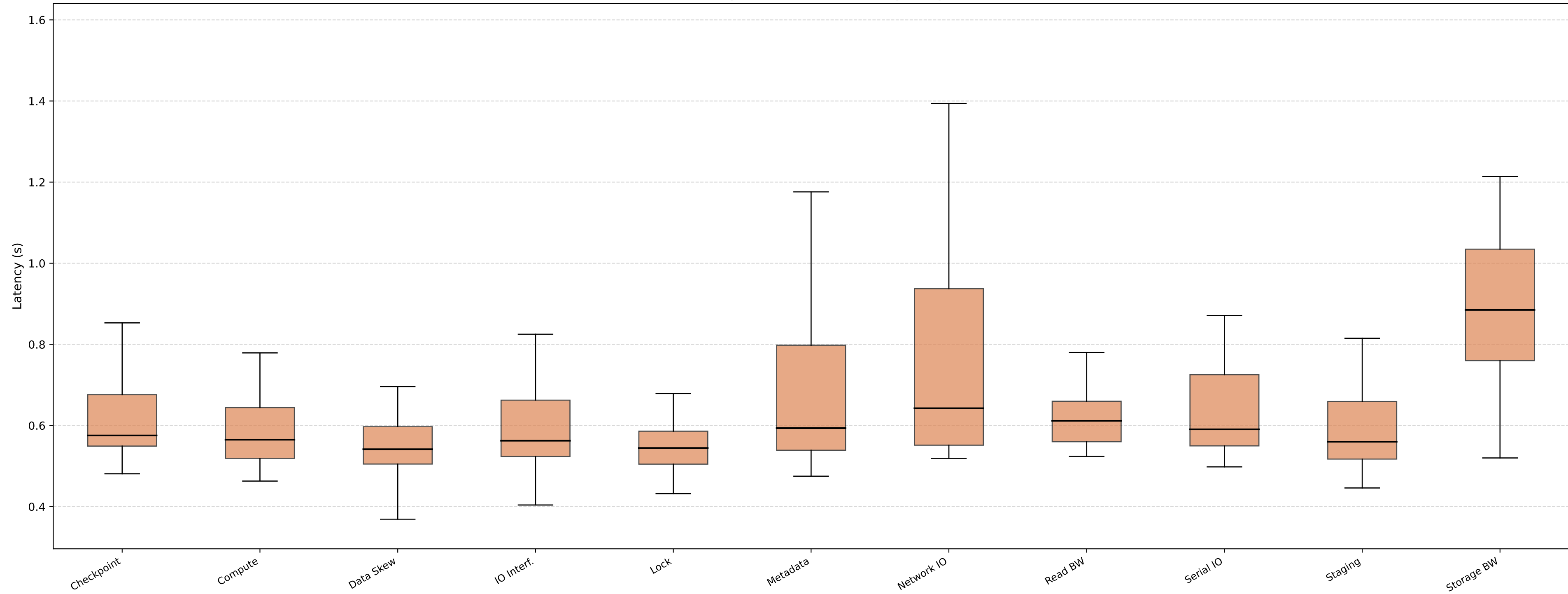
Latency per Class — Classify-Only
