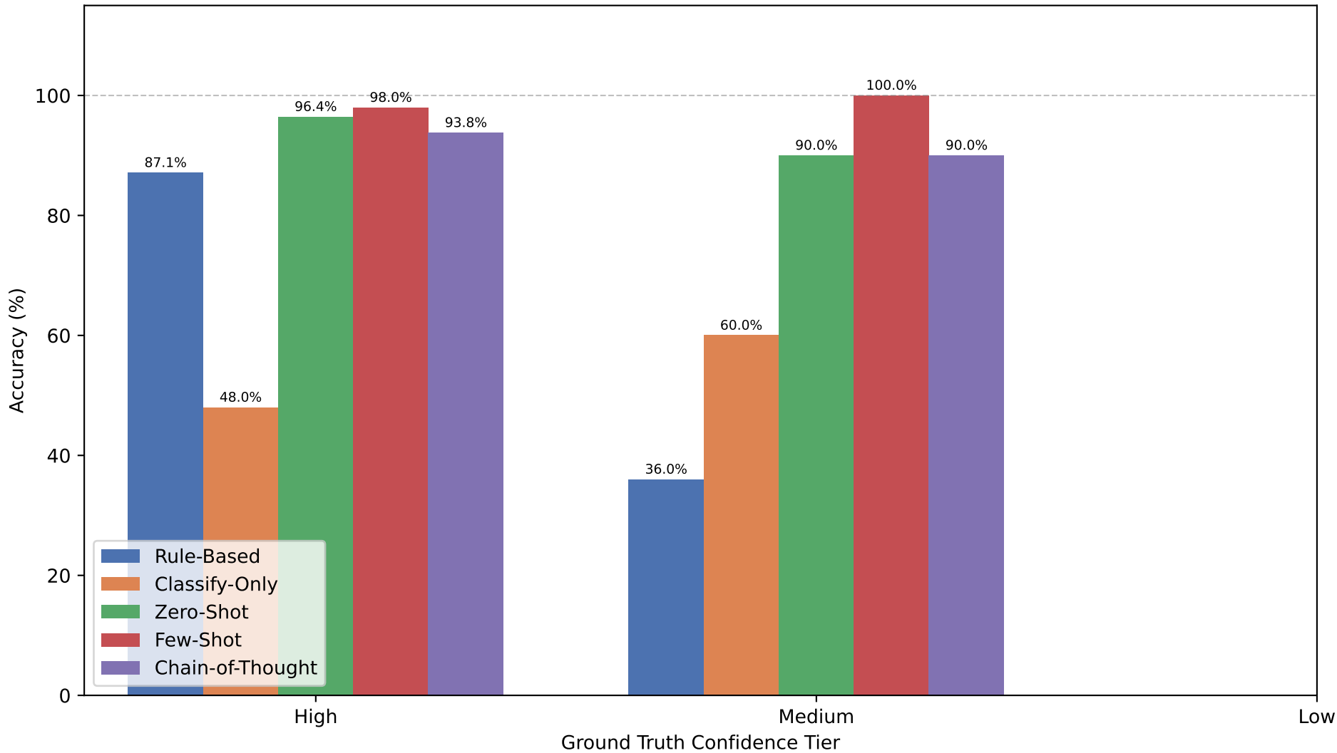
Accuracy by GT Confidence Tier — Claude Haiku 4.5
