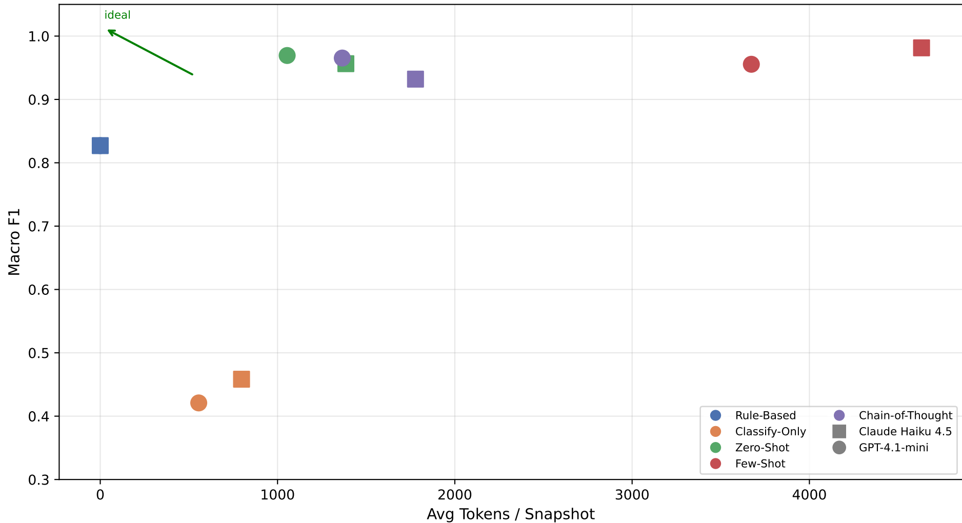
Cost vs. Accuracy Pareto — All Models (left = cheaper, up = better)
