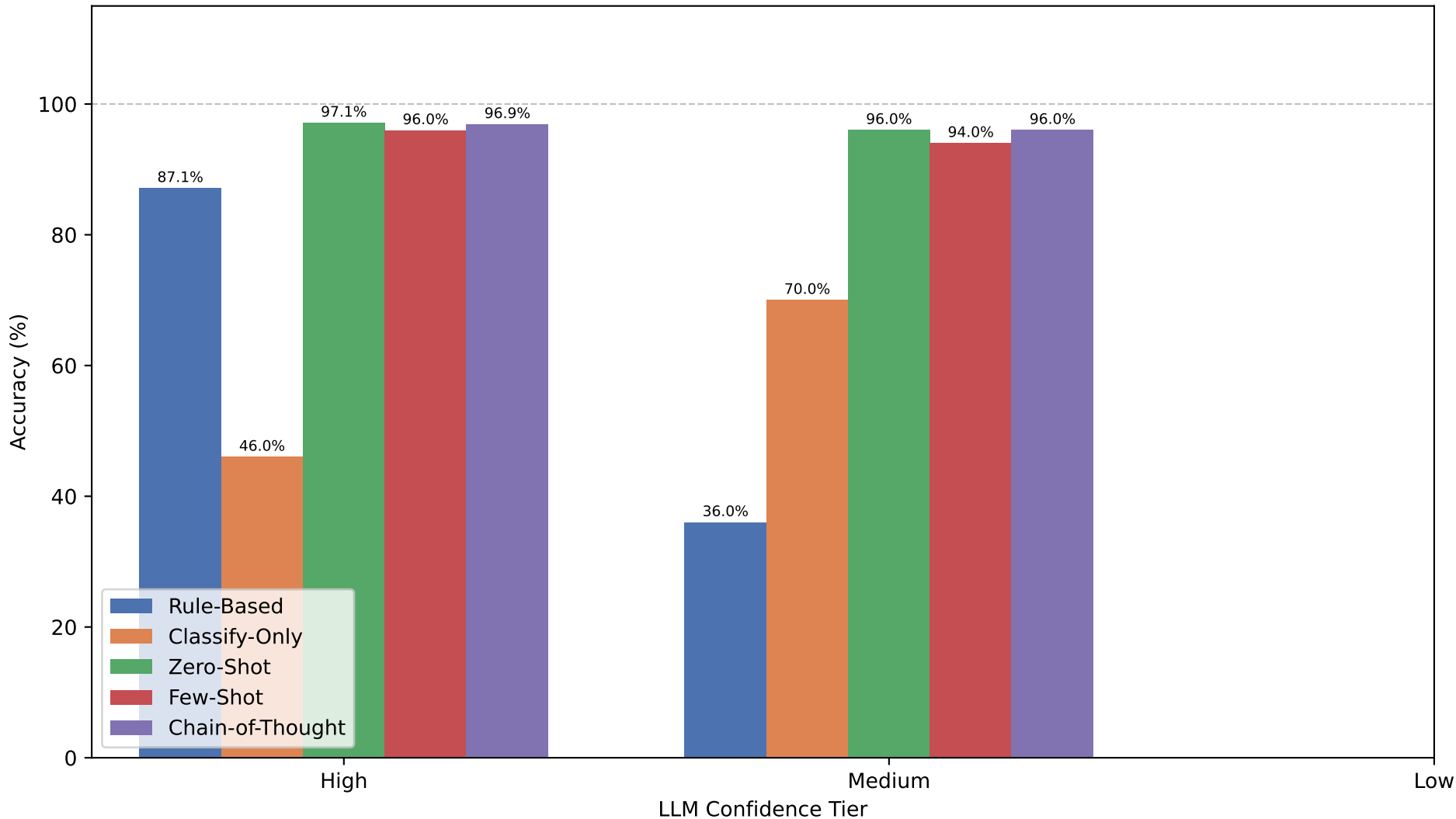
Accuracy by LLM Confidence Tier — GPT-4.1-mini
