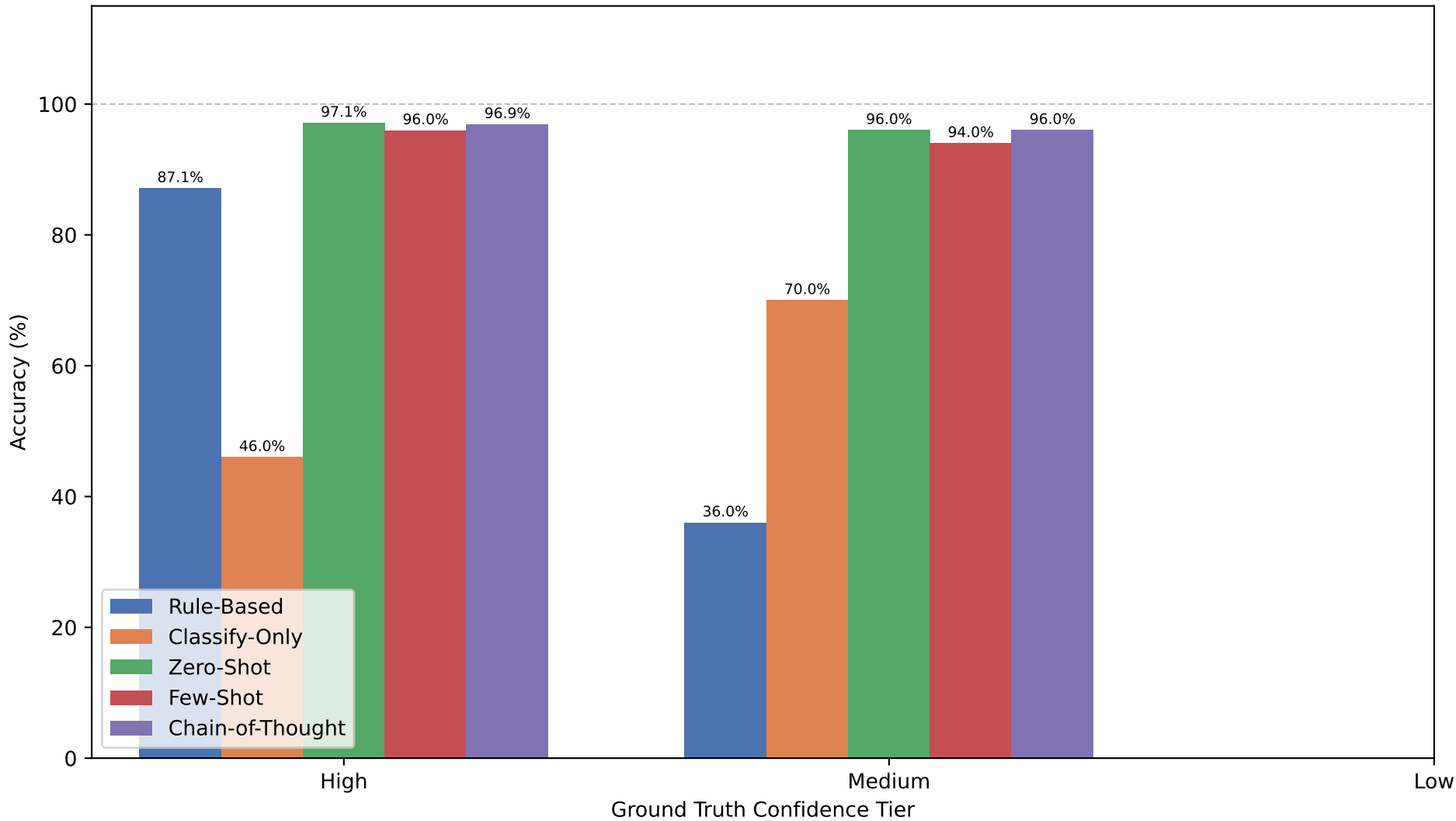
Accuracy by GT Confidence Tier — GPT-4.1-mini
