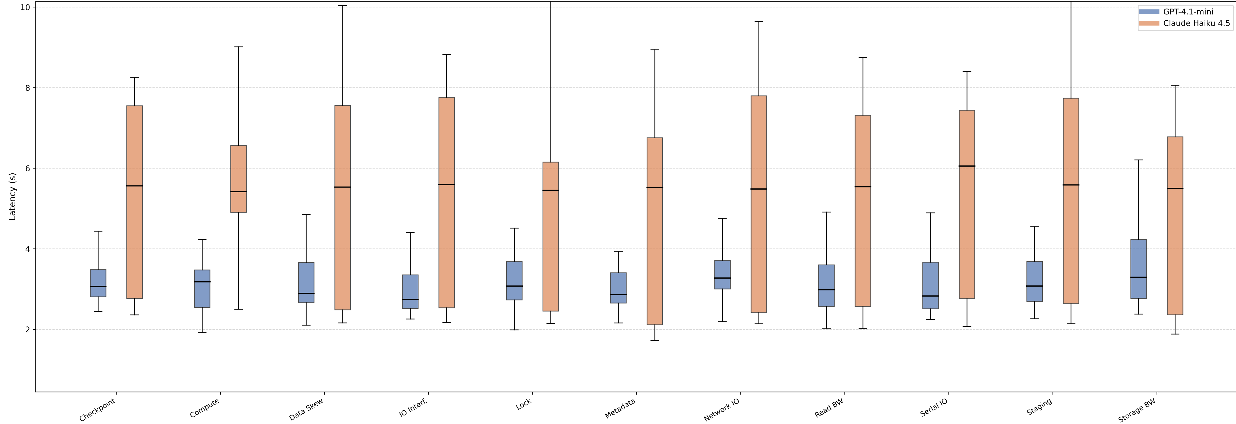
Latency per Class — Few-Shot
