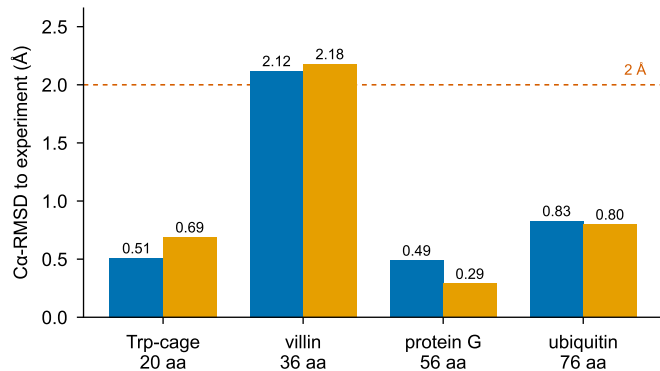
Single-sequence ESMFold vs. MSA-based AlphaFold2 on the four native sequences
