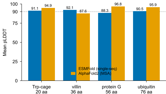
Single-sequence ESMFold vs. MSA-based AlphaFold2 on the four native sequences
