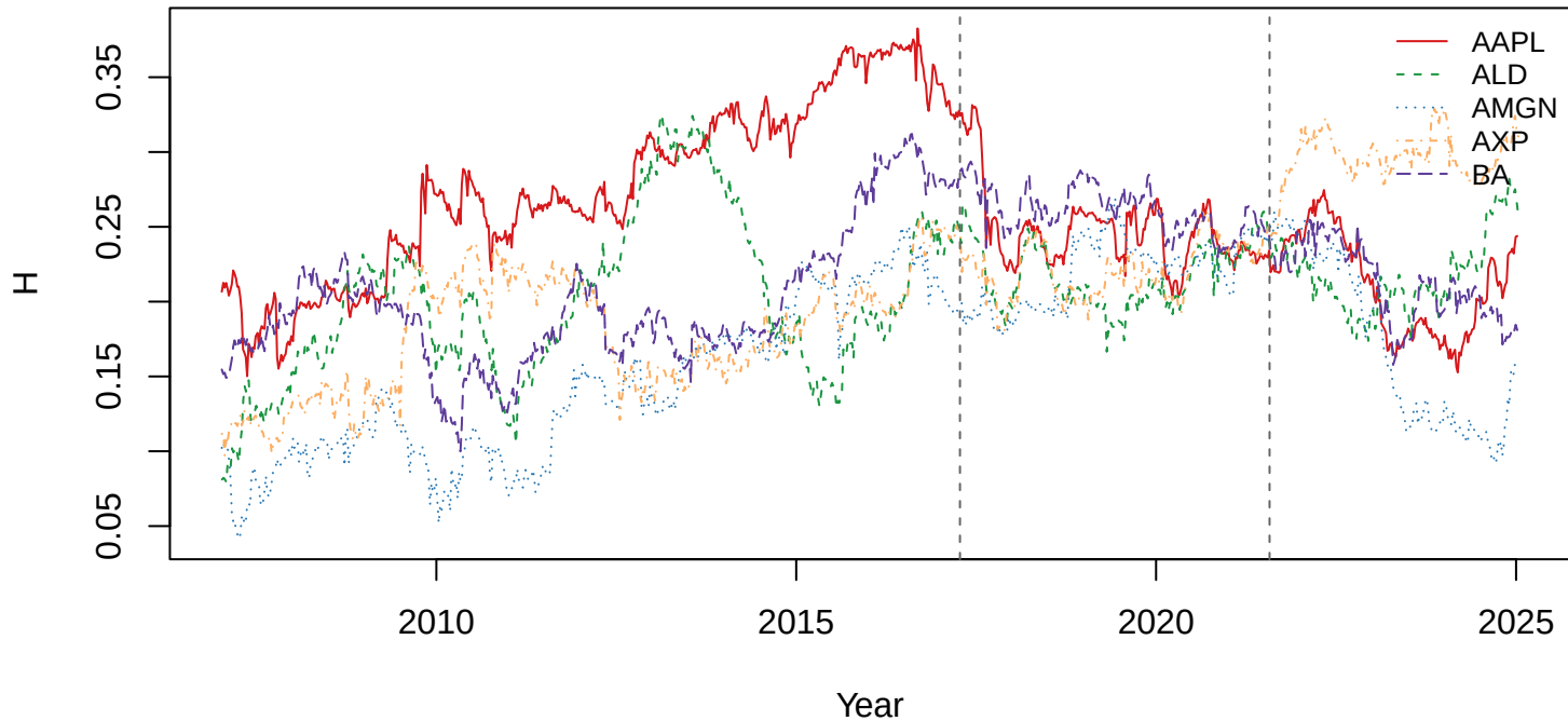
Rolling two-year estimates of H , log RV (DJ30 subset)
