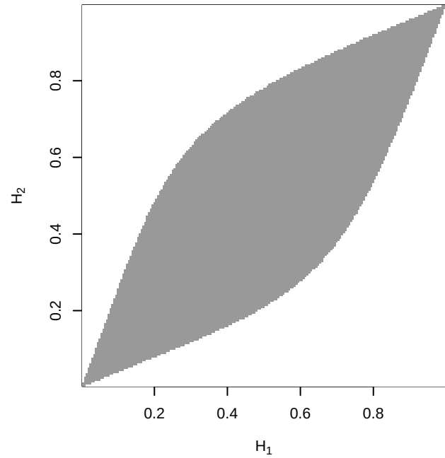
\rho = 0.9
