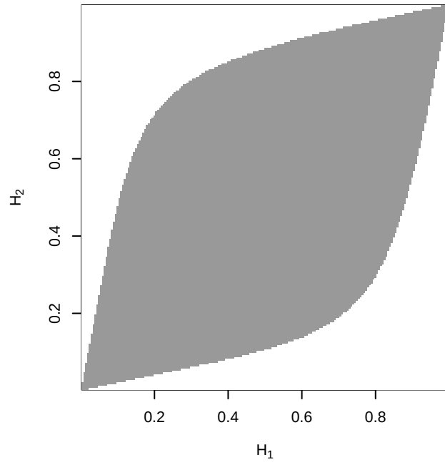
\rho = 0.75
