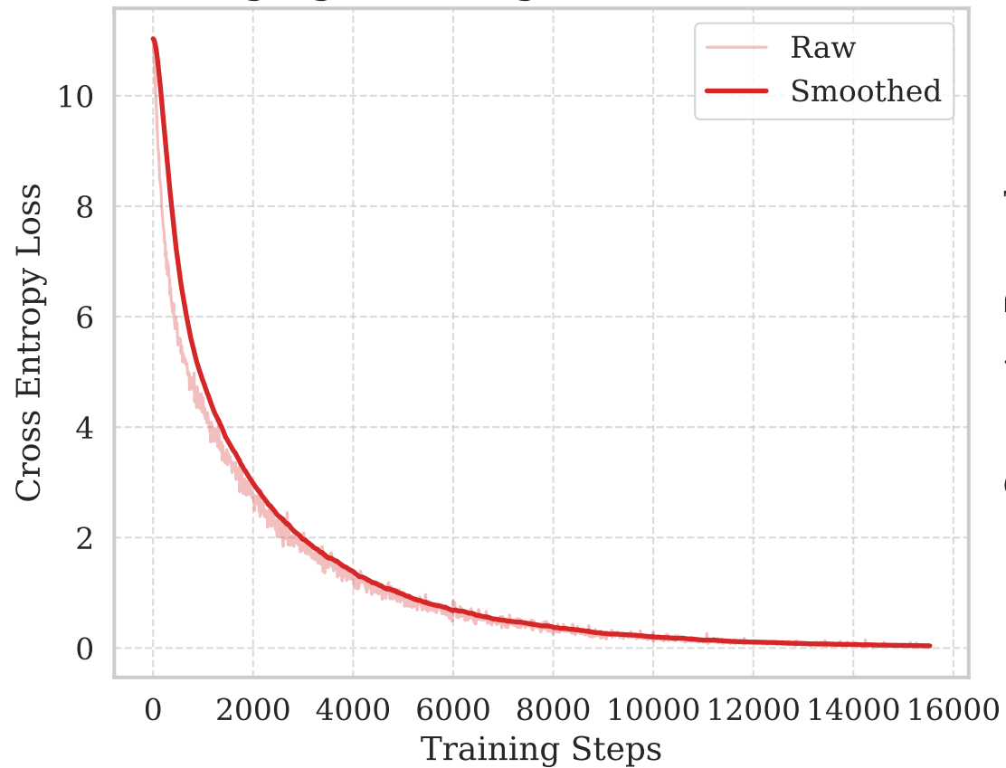
Language Modeling Loss (Wikitext-103)
