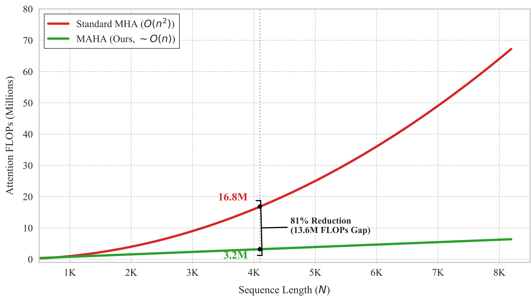
Figure 3. Attention FLOPs vs Sequence Length
