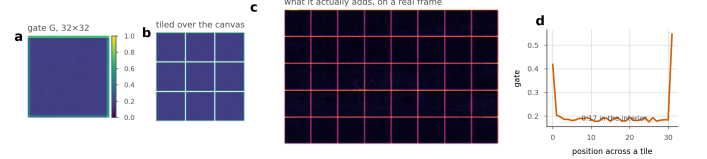
Figure 15. The deblocking gate, and what it does. a , the trained gate G , one scalar per position within a tile, shared across all 384 channels. b , the same gate tiled over the canvas, which is how it is applied. c , the correction it adds on a real frame: the tile lattice and nothing else. d , a cut through a tile. The gate reaches 0.76 at a corner and flattens at 0.17 rather than switching off.
