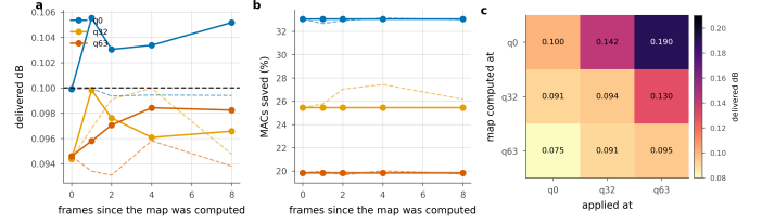
Figure 34. Reusing an exit map. Solid is the transferred map, dashed the one recomputed in place. a, b: reuse across frames of the same sequence. c: reuse across quality index; the entry is the delivered distortion against a 0.1 dB budget.
