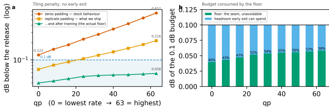
Figure 14. The tiling penalty across the whole rate range , every tile at full depth. The two steps that matter cost nothing, and the largest single factor is training the ladder with the seam present. Panel (b): the floor is charged inside the distortion budget and consumes a growing share of it.
