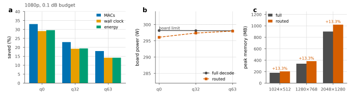
Figure 35. Three units for one saving. a, the same routed decode measured as arithmetic, as wall clock and as joules per frame, at 1080p and a 0.1 dB budget. Energy follows the clock, not the arithmetic. b, why: the board draws the same power either way, because the later groups run on a shrinking set of tiles and a partly idle GPU still draws its static power. c, peak memory, which routing raises rather than lowers, by 13.3% at every resolution that fitted on the card.
