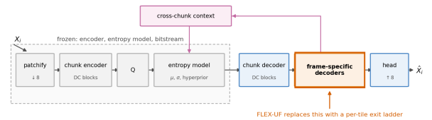
Figure 2. The decoder we modify , redrawn after DCVC-UF [14]. Everything left of the reconstruction stays frozen: the analysis transform, the entropy model and the coded payload. FLEX-UF replaces the frame-specific decoders with a ladder of exits taken per tile.
