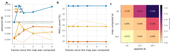
Figure 20. Reusing an exit map. Solid is the transferred map, dashed the one recomputed in place. a, b: reuse across frames of the same sequence. c: reuse across quality index; the entry is the delivered distortion against a 0.1 dB budget.
