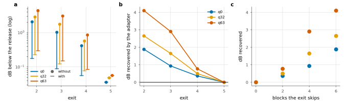
Figure 4. What the adapters are worth. a , each exit with and without its adapter. b , the dB the adapter recovers. c , the same against the number of blocks the exit skips, which is the design rationale measured.
