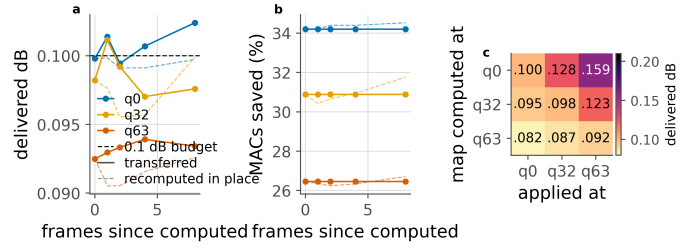
Figure 34. Reusing an exit map. Solid is the transferred map, dashed the one recomputed in place. a, b: reuse across frames of the same sequence. c: reuse across quality index; the entry is the delivered distortion against a 0.1 dB budget.
