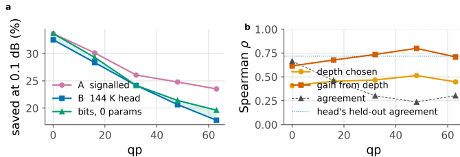
Figure 28. The calibrated bit rule. a, saving at 0.1 dB; shaded where the calibrated bit rule beats the trained head. b, what a tile's bit count is correlated with, against how often the rule agrees with the oracle outright; dotted is the head's own held-out agreement.
