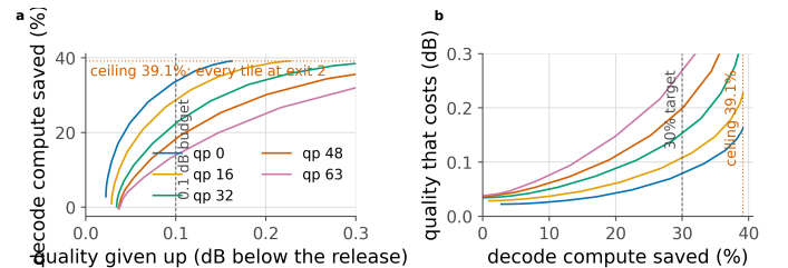
Figure 25. The trade-off, whole . a , what a budget buys, per rate; the dotted line is the arithmetic ceiling, 39.1%, and q_0 reaches it at 0.139 dB. b , the same relation inverted, so it reads as what a saving target costs. The three budgets reported elsewhere are three points on this curve.
