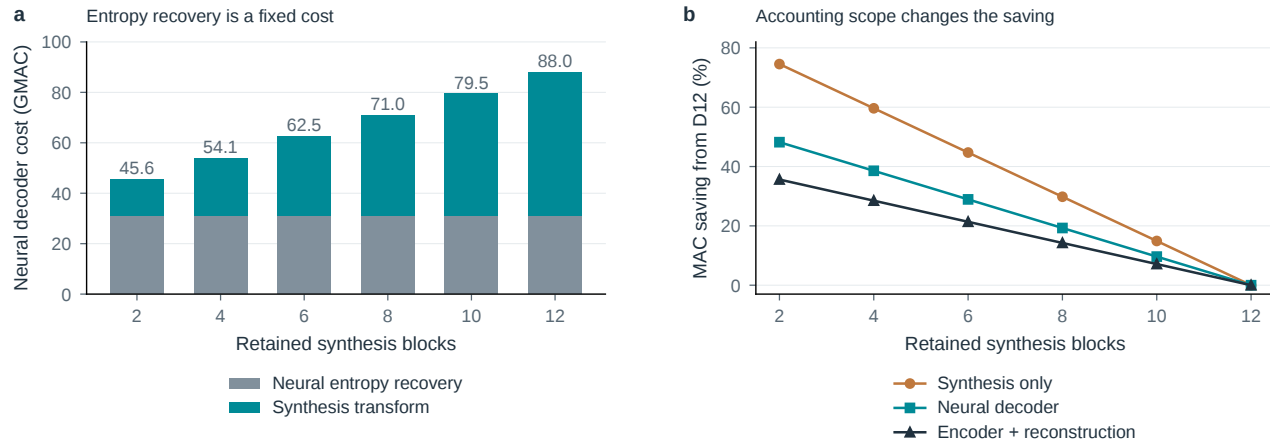
Figure S11. The arithmetic denominator changes the apparent saving. a , Synthesis varies with depth while neural entropy recovery stays fixed. b , The same architectural intervention under three accounting scopes. Counts use 512 \times 512 input and one MAC per multiply-accumulate; they are not observed kernel times. D8/D10 are architecture-only controls. Encoder totals include reconstruction but omit rANS, elementwise work, transfers and control overhead.
