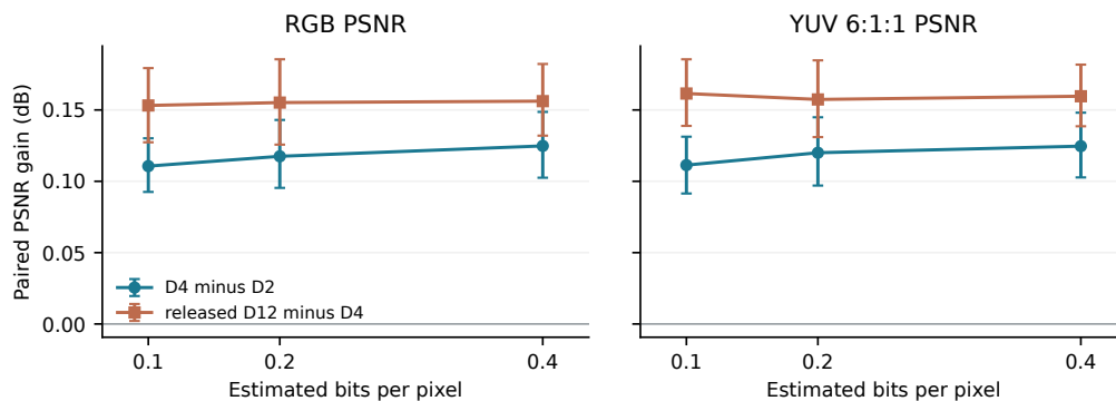
Figure S10. Completed D2/D4 codec quality at matched estimated rate. Image-paired PSNR differences on Kodak after the full 105-epoch official recipe, alongside the released D12 anchor. Rates are interpolated per image in log estimated bpp on common support. Bars show 95% paired-image bootstrap intervals ( n = 24 at 0.1/0.2 bpp; n = 23 at 0.4 bpp). YUV uses the upstream 6:1:1 metric. No actual-bitstream or same-recipe D12 result is implied.
