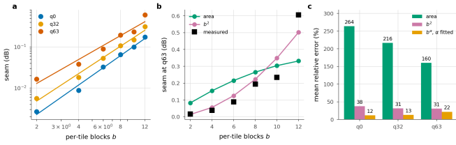
Figure 51. The seam against per-tile depth. a , the measurement with the fitted power law. b , both models against q63, one free scale each. c , mean relative error. The area fraction saturates once the border reaches every pixel and the penalty does not, which is where the area law fails as a predictor.
