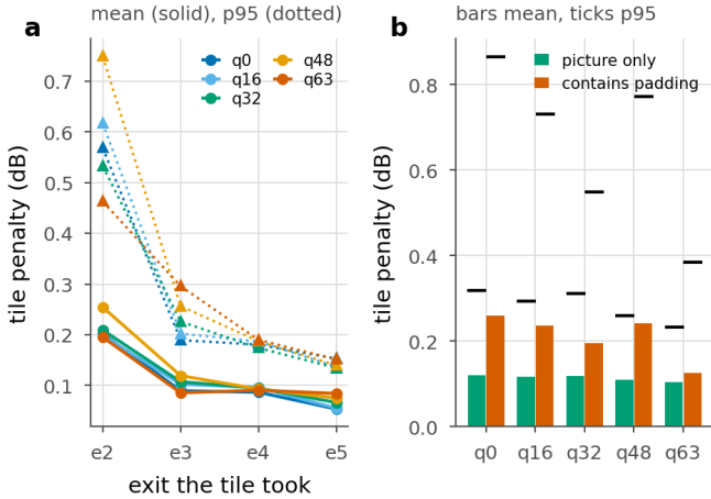
Figure 38. Where the tail comes from. a , mean and 95th percentile tile penalty against the exit the tile took. The tail sits on e2, the shallowest exit the clamp allows: at q0 its mean is 0.202 dB against 0.054 dB at e5, and all 79 tiles above 0.5 dB took it. b , the same penalty split by whether the tile contains replicated padding. A 1080p frame is padded to 2048x1280, so 200 of the bottom tile row's 256 rows are invented by replication, and those tiles carry roughly double the mean penalty at every rate: 0.261 dB against 0.121 dB at q0, and 65 of the 79 tiles above half a decibel are padded ones.
