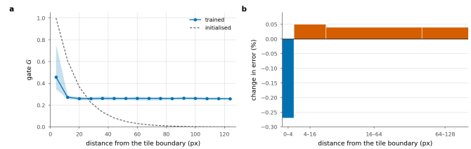
Figure 50. The learned deblocking filter, and where it wins. It is gated by position within a tile and applied once to the stitched frame, for 1.09% of the decode. a , the trained gate against distance from the boundary, beside its initialisation. b , the change in error by that distance; bar width is the share of pixels, so bar area is the contribution to the frame. It wins on the pixels nearest a boundary and loses on the rest, which is why a perfect gate still cannot pay for it.
