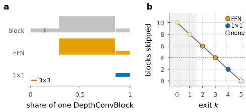
Figure 27. Inside an exit adapter. a , one DepthConvBlock and the two adapters, drawn to scale: bar length is a share of the block, bar height the channel width written. Neither adapter contains the block's only 3×3 (the hairline rule), so neither adds receptive field or seam penalty, which is the design constraint the seam measurement imposes. b , blocks skipped per exit, coloured by adapter; the rule switches to the FFN at four skipped blocks. Lengths are counted with hooks off the modules themselves.
