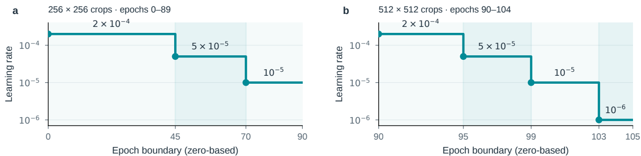
Figure S9. The full official schedule is retained. a , First 90 epochs with 256^2 crops. b , Final 15 epochs with 512^2 crops, on a separately expanded epoch axis. Zero-based boundaries delimit the seven learning-rate stages; the protocol applies to D2/D4/D6. These are prescribed settings, not learning curves.
