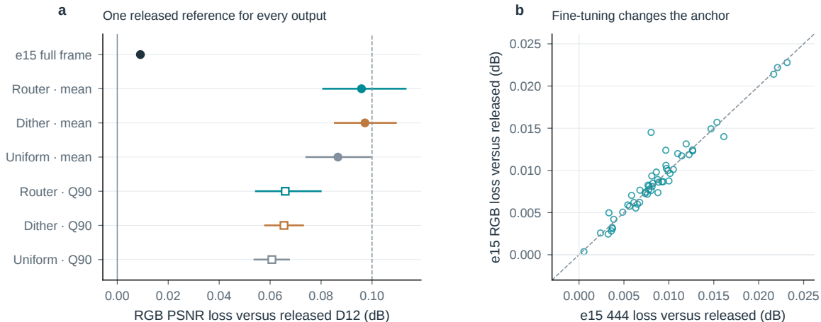
Figure S21. Measure the anchor before interpreting the loss budget. The same 53 first frames, QP32, valid-pixel support and CPU FP32 reconstruction. a , e15 full-frame and six fixed policies relative to released D12; points and intervals show means and paired 95% sequence-bootstrap intervals. Filled circles use mean control and hollow squares Q90; the dark full-frame point measures anchor drift. The dashed 0.1 dB line is a numerical reference. b , Per-sequence e15 drift under equal-channel unclipped 444 and converted/clipped RGB. The diagonal denotes metric agreement. No output or policy is reselected when the reference changes.
