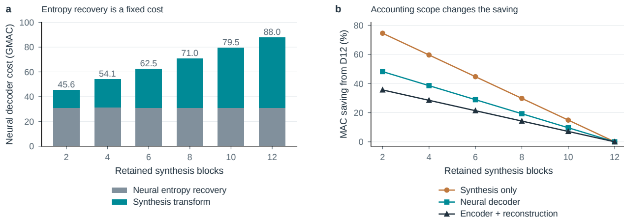
Figure S10. The arithmetic denominator changes the apparent saving. a , Synthesis varies with depth while neural entropy recovery stays fixed. b , The same architectural intervention under three accounting scopes. Counts use 512 \times 512 input and one MAC per multiply-accumulate; they are not observed kernel times. D8/D10 are architecture-only controls. Encoder totals include reconstruction but omit rANS, elementwise work, transfers and control overhead.
