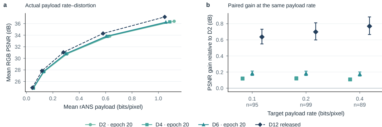
Figure S19. Shallow models are close, but not identical, at equal coded rate. a , Mean RGB PSNR and actual payload over all 100 crops at five QPs; joining lines are visual guides. b , Per-image interpolation and paired differences on four-model common support, with 95% image-bootstrap intervals. D2/D4/D6 are frozen epoch-20 models; released D12 is not matched in training history. These measured streams establish an interim CPU rate–distortion comparison, not final quality or native runtime.
