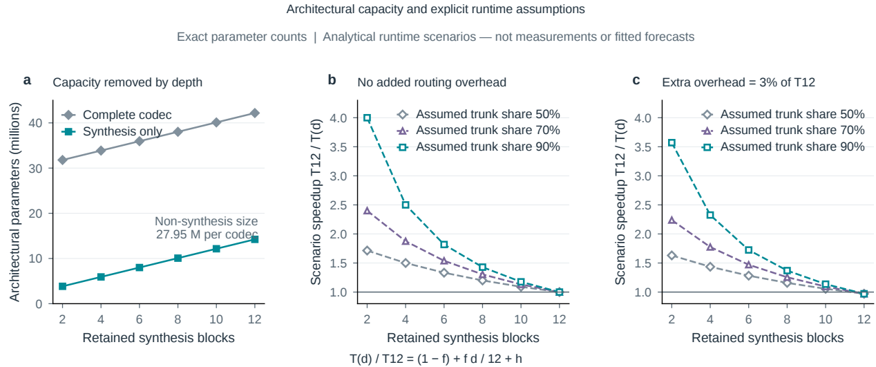
Figure S25. A transparent design-space illustration for unfinished experiments. a , Exact architectural parameter counts. b,c , Analytical runtime sensitivity to assumed trunk-time share and added overhead. Open markers and dashed lines denote assumptions, not measurements or fitted forecasts. No quality or bitrate outcome is assigned to an unfinished model.
