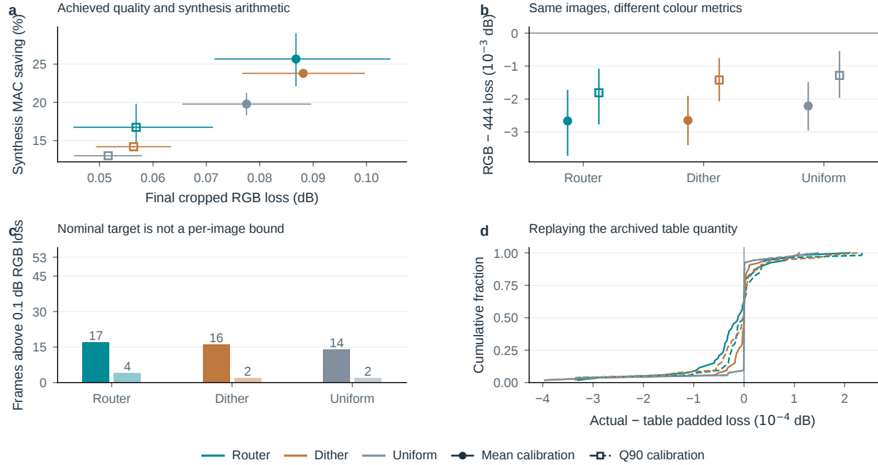
Figure S27. Carry the fixed decision through to the actual image. All 53 sequences at QP32, with no outcome-based exclusions. a , Achieved RGB loss and synthesis MAC saving with conditional 95% sequence-bootstrap intervals; these points are not an equal-quality frontier. b , RGB-minus-444 loss on the same support and reference. c , Counts above the nominal numerical threshold; pale bars denote Q90 calibration. d , Actual-minus-table loss on padded support. Mean and Q90 controls use a different calibration reference and metric from the cropped RGB report. The paired router-dither saving intervals include zero under both controls.
