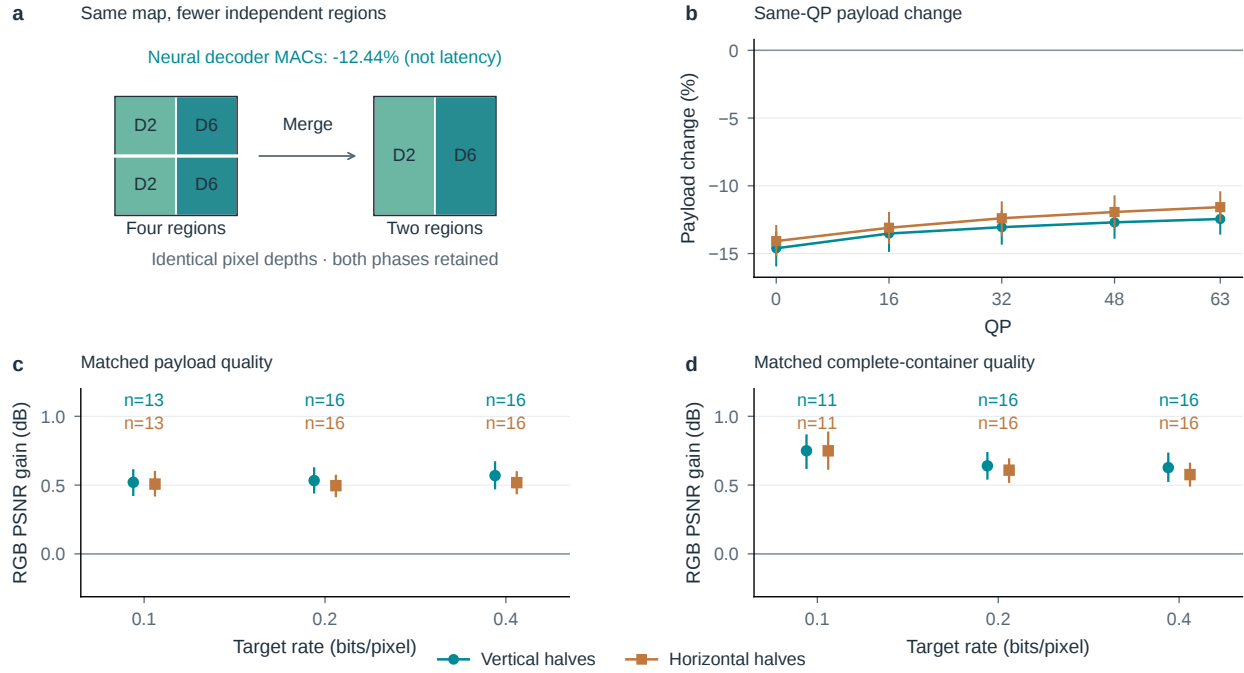
Figure S34. Better region execution without a better selector. a , One phase of the fixed depth-map control; every pixel keeps its D2 or D6 assignment. b , Same-QP relative payload change after coalescing. c,d , RGB PSNR gain at matched payload and complete-container rate, on shared vertical scales. Complementary phases are averaged within image before 95% paired-image bootstrap intervals. Counts show the common support of both phases and implementations, without extrapolation. The 800 outputs include unmerged checkerboards; those have no adjacent same-depth regions to combine. CPU FP32 research streams and epoch-20 weights are used throughout; this is neither learned routing nor a runtime benchmark.
