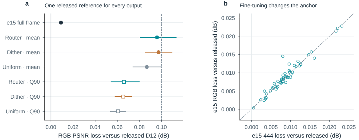
Figure S28. Measure the anchor before interpreting the loss budget. The same 53 first frames, QP32, valid-pixel support and CPU FP32 reconstruction. a , e15 full-frame and six fixed policies relative to released D12; points and intervals show means and paired 95% sequence-bootstrap intervals. Filled circles use mean control and hollow squares Q90; the dark full-frame point measures anchor drift. The dashed 0.1 dB line is a numerical reference. b , Per-sequence e15 drift under equal-channel unclipped 444 and converted/clipped RGB. The diagonal denotes metric agreement. No output or policy is reselected when the reference changes.
