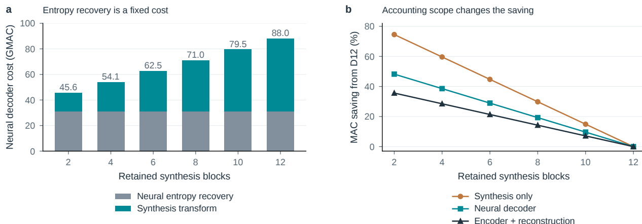
Figure S18. The arithmetic denominator changes the apparent saving. a , Synthesis varies with depth while neural entropy recovery stays fixed. b , The same architectural intervention under three accounting scopes. Counts use 512 \times 512 input and one MAC per multiply-accumulate; they are not observed kernel times. D8/D10 are architecture-only controls. Encoder totals include reconstruction but omit rANS, elementwise work, transfers and control overhead.
