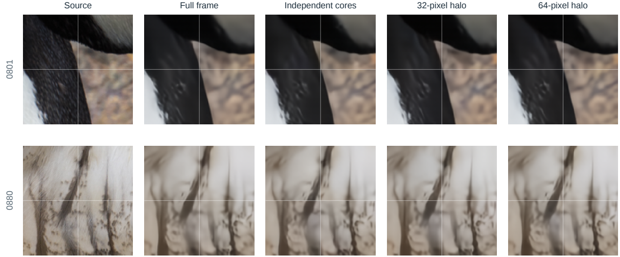
Figure S32. Predeclared views at the region intersection. D6 epoch 20, QP32, DIV2K 0801 and 0880. All panels use rows and columns 192:320 of the same 512-square crop; images and window were fixed before outcomes. The common light cross marks the patch boundary. Display images are rounded to 8 bit; numerical metrics use floating-point RGB. These are same-QP views, not equal-bitrate reconstructions.
