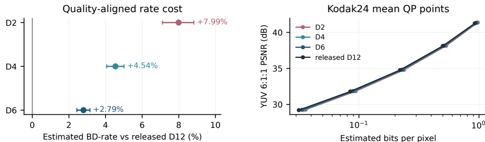
Figure S17. The completed independent codecs approach the release as depth grows. Left, per-image YUV 6:1:1 BD-rate cost on the four-model common PSNR interval; bars are 95% paired-image bootstrap intervals ( n = 24 ). Right, mean five-QP operating points on Kodak24. Rates are deterministic entropy estimates, not actual bitstreams. Released D12 differs in training history from the three scratch models.
