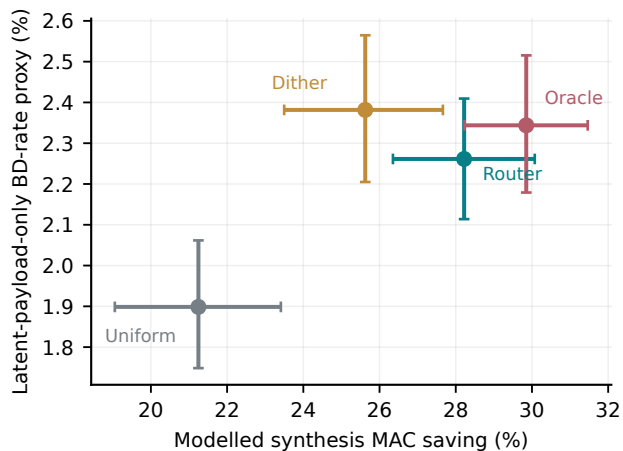
d Rate-computation trade-off
