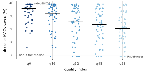
Figure 18. What the set mean hides. Every test sequence as a point, at the 0.1 dB budget; the bar is the median. At the lowest rate the saving runs from 6.0% to 39.1% across the 53 sequences and at the highest from -1.0% to 39.1%. The spread within a rate is larger than the difference between rates, and it is content, not noise: the same sequences sit at the same end of it at every rate.
