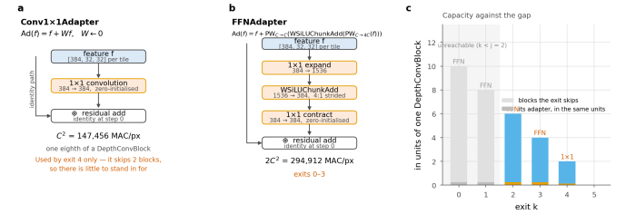
Figure 2. Inside an exit adapter. Both kinds are entirely pointwise, so no adapter adds receptive field and none of them contributes any tile-boundary penalty. Capacity is matched to the number of blocks the exit skips, and the adapter’s own cost is charged against the saving, so an exit-2 tile saves six blocks minus 0.25.
