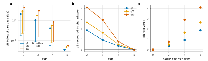
Figure 3. What the adapters are worth. a, each exit with and without its adapter. b, the dB the adapter recovers. c, the same against the number of blocks the exit skips, which is the design rationale measured.
