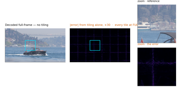
Figure 4. The artefact, before anything is done about it. One frame decoded twice from the same bitstream with the same weights, every tile at full depth, stock zero padding, and no early exit anywhere. The only difference is that the right-hand decode was tiled. The error map is the tile lattice and nothing else.
