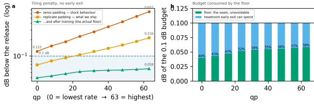
Figure 6. The tiling penalty across the whole rate range , every tile at full depth. The two steps that matter cost nothing, and the largest single factor is training the ladder with the seam present. Panel (b): the floor is charged inside the quality budget and consumes a growing share of it.
