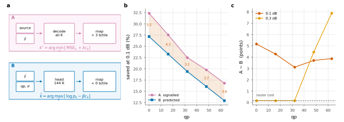
Figure 16. Who decides. (a) A holds the source, so it can decode all K exits per tile and pick the true minimiser; it signals the map at \sim 89 bits/frame. B never sees the source and signals nothing; its 144 K-parameter head reads \hat{y} , the entropy scales and qp . (b) Saving at 0.1 dB; shading is what a bit-exact bitstream costs. (c) That cost is smallest at q32, where the tilt needed to move the router off its training multiplier is essentially zero, and grows in both directions. At 0.3 dB it collapses to the router's own 0.163% wherever the budget saturates the ladder, and widens where it does not.
