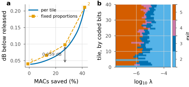
Figure 44. The two achievable sets, on one frame. a , the per-tile frontier of Theorem 4 traced by sweeping \lambda , against the fixed-proportion chain of Proposition 3 through the four uniform-depth points, labelled by exit. The per-tile curve lies below the chain everywhere between the vertices, by 0.059 dB at the exit-3 vertex. b , the exit each of the 40 tiles takes as \lambda rises, tiles ordered by the bits the entropy coder spent on them. Every row is non-increasing, which is Proposition 2 per tile, and the rows differ, which is what Theorem 4 buys over Proposition 3. The bottom row is a tile that never leaves the shallowest exit.
