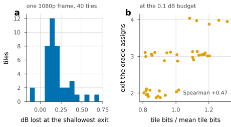
Figure 3. Why depth should not be uniform. One 1080p frame, 40 tiles. a , what each tile loses if it stops at the shallowest exit the ladder allows: a few lose nothing measurable and one loses 0.71 dB. A single depth for the frame has to be set by the worst of them. b , the bits the entropy model has already spent on a tile against the exit the Lagrangian oracle sends it to, at the 0.1 dB budget. The signal the decoder needs is already in the file.
