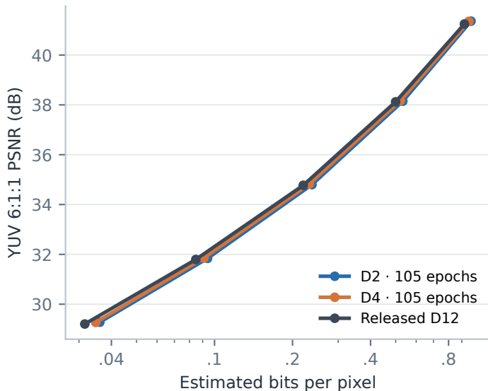
a Final codec curves · Kodak, n = 24
