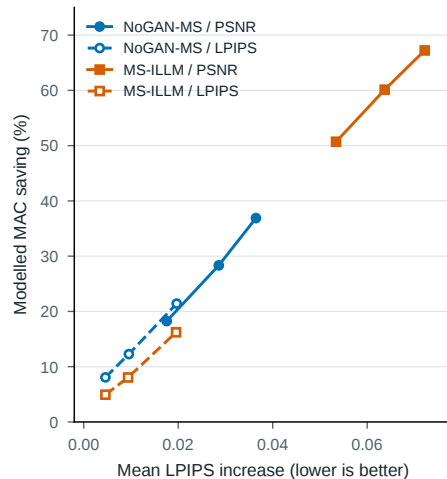
b PSNR permits perceptual loss
