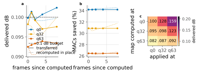
Figure 28. Reusing an exit map. Solid is the transferred map, dashed the one recomputed in place. a, b: reuse across frames of the same sequence. c: reuse across quality index; the entry is the delivered distortion against a 0.1 dB budget.
