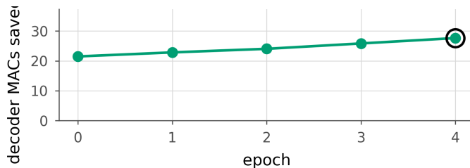
Figure 31. The run had not converged. Measured saving at the 0.1 dB budget on the 53 test frames, hook-counted, one point per completed epoch of the reported run. The circled point is the checkpoint this paper reports. The training loss over the same epochs is flat; the supplement shows the two together.
