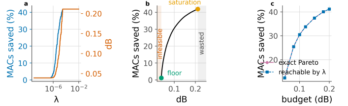
Figure 21. The structure of the allocation, on one frame. a, compute and distortion are monotone in the multiplier. b, the frontier, with both ends and both dead bands marked on the panel. c, what the Lagrangian reaches against the exact Pareto set, enumerated by dynamic programming.
