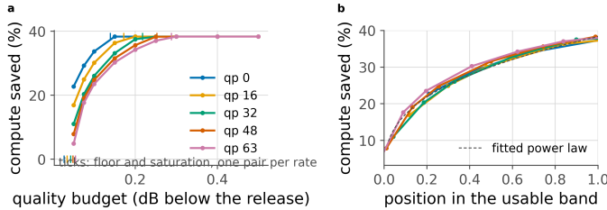
Figure 22. The band is the rate dependence. a , saving against the budget, with each rate's floor and saturation point ticked. b , the same with the budget axis rescaled onto each rate's own band. Five curves become one; dashed is the one-parameter power law fitted to all of them.
