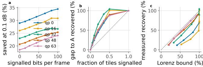
Figure 27. Partial signalling. a, saving against the bits spent on the map; each line runs from B on the left to A on the right. b, the same normalised by the A-to-B gap; dashed is proportional recovery. c, against the fixed- \lambda Lorenz bound; points above the dashed line are allocations one multiplier cannot reach.
