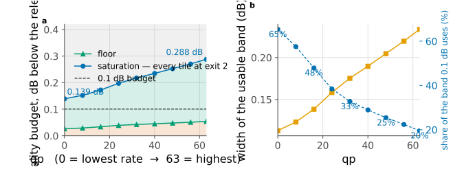
Figure 20. Three regions, and only the middle one is a design choice. Below the floor no allocation meets the budget; above saturation every tile already takes the cheapest exit. The 0.1 dB budget uses 65% of the band at the lowest rate and 20% at the highest.
