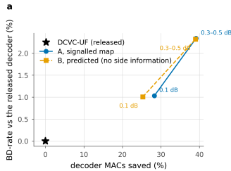
Figure 30. What the saving costs in rate. BD-rate against the released decoder, against the decoder MACs saved, for both configurations at the three budgets; each point is labelled with the budget that produced it. The star is the released decoder itself: no saving, no cost. Anchored on the same bitstream, so a BD-rate here is the price of decoding one file with fewer operations, not one codec against another.
