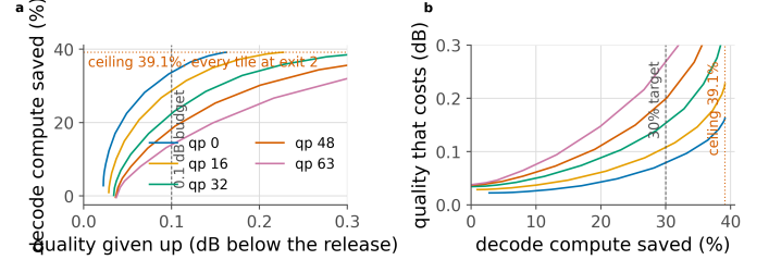
Figure 23. The trade-off, whole. a , what a budget buys, per rate; the dotted line is the arithmetic ceiling, 39.1%, and q0 reaches it at 0.139 dB. b , the same relation inverted, so it reads as what a saving target costs. The three budgets reported elsewhere are three points on this curve.
