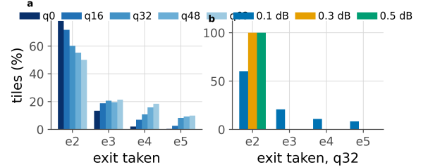
Figure 16. Where the ladder is used. Tiles per exit over the whole test set. a , the 0.1 dB budget at five rates. b , one rate at the three budgets. Exits below the split depth do not exist and are not drawn.
