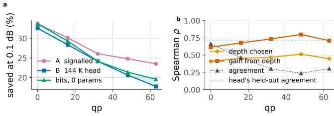
Figure 25. The calibrated bit rule. a , saving at 0.1 dB; shaded where the calibrated bit rule beats the trained head. b , what a tile's bit count is correlated with, against how often the rule agrees with the oracle outright; dotted is the head's own held-out agreement.
