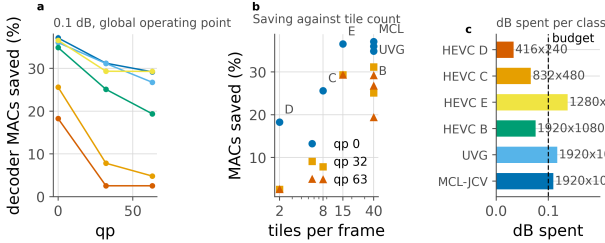
Figure 19. Saving by test class at one global operating point. \lambda is bisected once so the whole set lands on the budget, exactly as it would be in deployment; each class is then reported at that \lambda . The ordering follows tile count, not content.
