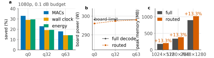
Figure 29. Three units for one saving. a, the same routed decode measured as arithmetic, as wall clock and as joules per frame, at 1080p and a 0.1 dB budget. Energy follows the clock, not the arithmetic. b, why: the board draws the same power either way, because the later groups run on a shrinking set of tiles and a partly idle GPU still draws its static power. c, peak memory, which routing raises rather than lowers, by 13.3% at every resolution that fitted on the card.
