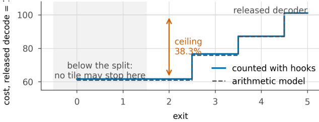
Figure 41. The ladder, priced. What a tile costs at each exit, as a percentage of one released decode, counted with hooks on the executed pass and beside the arithmetic model the argmin uses. Exits below the split depth are not distinct, because the first j groups run for every tile whatever it does. The deepest exit costs slightly more than the release, which is the full-frame deblocking pass. Reported savings in the paper are the hook count.
