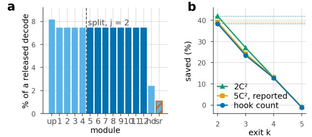
Figure 40. Where the arithmetic is, and what an exit saves. a , one released decode by module: the opening upsample, the twelve trunk blocks, the head, and the seam-repair pass this work adds (hatched). Light bars always run; dark bars are the eight blocks after the split that a tile can skip. b , the saving at each reachable exit under three prices for the same architecture, with each price's ceiling dotted. Section B.5 is the table behind it.
