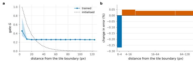
Figure 62. The learned deblocking filter, and where it wins. It is gated by position within a tile and applied once to the stitched frame, for 1.09% of the decode. a , the trained gate against distance from the boundary, beside its initialisation. b , the change in error by that distance; bar width is the share of pixels, so bar area is the contribution to the frame. It wins on the pixels nearest a boundary and loses on the rest, which is why a perfect gate still cannot pay for it.
