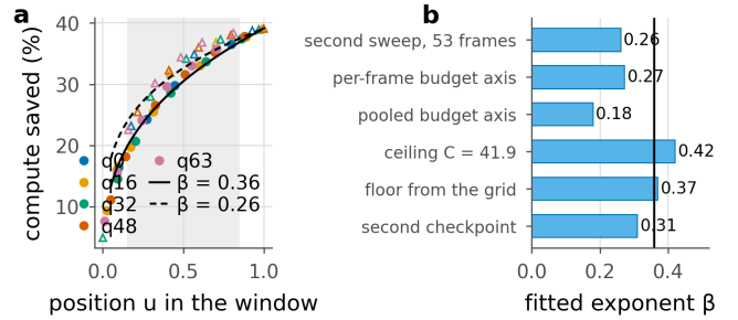
Figure 56. The collapse, and what the exponent is sensitive to. a , the rescaled points from two sweeps of the pinned checkpoint, filled circles for the 106-frame grid and open triangles for the 53-frame frontier, with the power law fitted to each over the shaded window. The two sweeps of one checkpoint do not lie on one curve. b , the exponent under one change at a time, with the vertical line at the exponent of the first row of Table 75. The change of checkpoint, which the main paper reads as a finding, is the smallest of the six.
