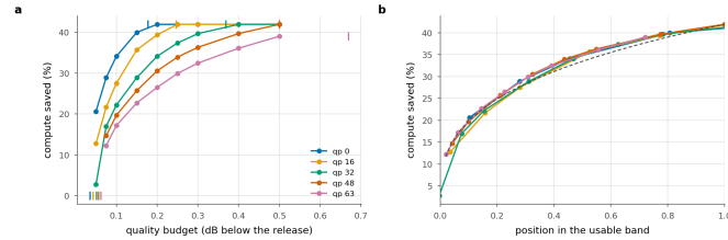
Figure 54. The collapse on the second training run. a , saving against budget, one line per rate, with each rate's floor and saturation point ticked. b , the same with the budget axis rescaled to each rate's own window; dashed is the one-parameter power law. The main paper shows this pair for the pinned checkpoint.
