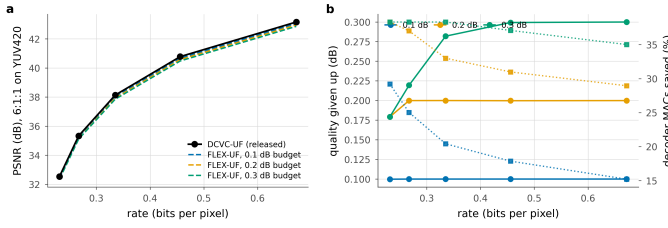
Figure 48. a , rate against quality over the five quality indices, the released DCVC-UF intra decoder and FLEX-UF at three budgets, on the 53 CTC intra frames. Both axes come from one pass over the same frames, and the encoders are asserted bit-identical on the weights before a shared rate is reported, because a shared x-axis is a claim rather than a convenience. b , the same difference magnified: the decibels each budget delivered, against the decoder arithmetic it bought on the right-hand axis.
