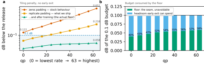
Figure 53. The tiling penalty across the whole rate range, every tile at full depth, so this is the floor and nothing else. a , the steps that reduce it, of which the two that matter cost no arithmetic; the largest single factor is training the ladder with the seam present. b , the floor as a share of the 0.1 dB budget: it is charged inside the budget and consumes a growing part of it as the rate rises, which is one of the two reasons the saving falls with rate.
