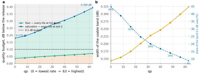
Figure 52. Three regions, and only the middle one is a design choice. Below the floor no allocation meets the budget; above saturation every tile already takes the cheapest exit and a looser budget buys nothing. The 0.1 dB budget uses 45% of the band at the lowest rate and 9% at the highest, which is why the same budget behaves so differently at the two ends of the rate range.
