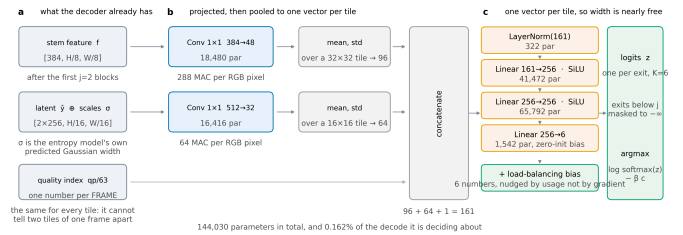
Figure 58. The router head. a, the three things it reads, all already held by the decoder at the moment the decision is needed. b, each projected by a 1 \times 1 , then reduced to one vector per tile by its mean and standard deviation. c, a three-layer perceptron, one pass per tile. Every shape and parameter count in the figure is read off the module when the figure is drawn.
