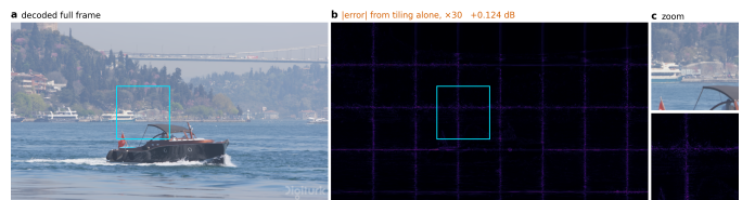
Figure 61. The seam, at frame scale. a, the decoded frame. b, the absolute error against a full-frame decode of the same latent, amplified 30×, with every tile at the deepest exit so that nothing here is early exiting. c, a zoom on one junction. The tile grid is the error: 0.124 dB at q63, paid before the allocation begins.
