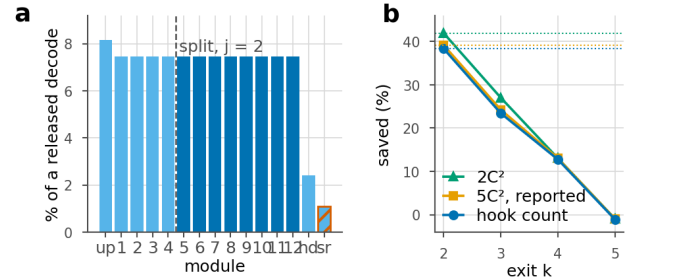
Figure 42. Where the arithmetic is, and what an exit saves. a , one released decode by module: the opening upsample, the twelve trunk blocks, the head, and the seam-repair pass this work adds (hatched). Light bars always run; dark bars are the eight blocks after the split that a tile can skip. b , the saving at each reachable exit under three prices for the same architecture, with each price's ceiling dotted. Section B.5 is the table behind it.
