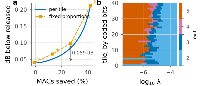
Figure 46. The two achievable sets, on one frame. a , the per-tile frontier of Theorem 4 traced by sweeping \lambda , against the fixed-proportion chain of Proposition 3 through the four uniform-depth points, labelled by exit. The per-tile curve lies below the chain everywhere between the vertices, by 0.059 dB at the exit-3 vertex. b , the exit each of the 40 tiles takes as \lambda rises, tiles ordered by the bits the entropy coder spent on them. Every row is non-increasing, which is Proposition 2 per tile, and the rows differ, which is what Theorem 4 buys over Proposition 3. The bottom row is a tile that never leaves the shallowest exit.
