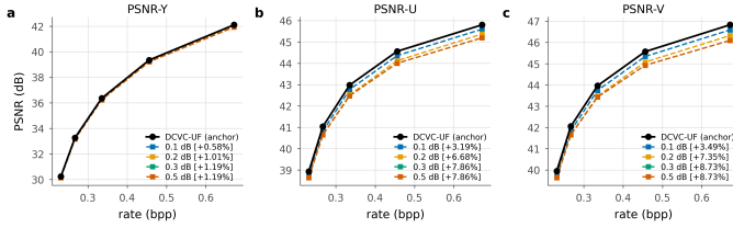
Figure 63. Rate-distortion per colour component , ours against the released decoder, one panel per component, with each budget's BD-rate against the anchor in brackets. The anchor is the released decoder on the same bitstream, so a bracket is the price of decoding one file with fewer operations rather than one codec against another.
