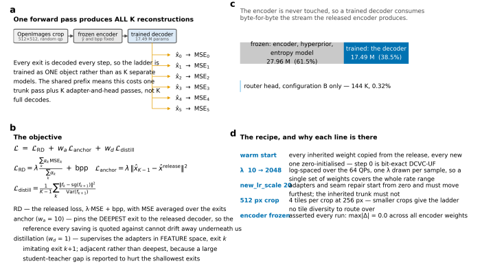
Figure 41. The training scheme. a, one forward pass produces all K reconstructions, so the ladder is trained as one object. b, the three loss terms. c, the encoder is never touched. d, why each line of the recipe is there. The figure is a schematic drawn from the model definition; the parameter counts it carries are the ones tabulated in A.5.
