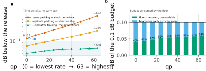
Figure 55. The tiling penalty across the whole rate range, every tile at full depth, so this is the floor and nothing else. a , the steps that reduce it, of which the two that matter cost no arithmetic; the largest single factor is training the ladder with the seam present. b , the floor as a share of the 0.1 dB budget: it is charged inside the budget and consumes a growing part of it as the rate rises, which is one of the two reasons the saving falls with rate.
