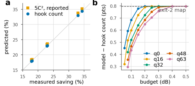
Figure 44. The model against the meter. a, six decodes at two resolutions: the hook-count assembly lies on the identity line and the model the paper reports lies above it. b, the same residual over the whole budget grid, 9 budgets by 5 quality indices on 53 sequences. It is positive everywhere, grows with the budget, and saturates at the value an all-exit-2 map implies.
