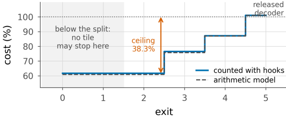
Figure 43. The ladder, priced. What a tile costs at each exit, as a percentage of one released decode, counted with hooks on the executed pass and beside the arithmetic model the argmin uses. Exits below the split depth are not distinct, because the first j groups run for every tile whatever it does. The deepest exit costs slightly more than the release, which is the full-frame deblocking pass. Reported savings in the paper are the hook count.
