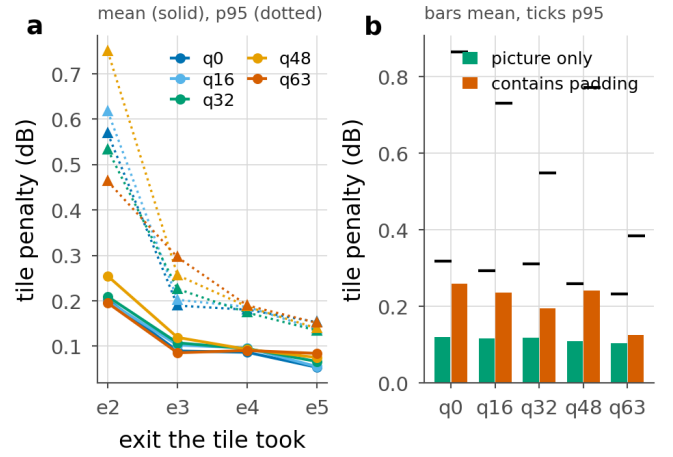
Figure 52. Where the tail comes from. a , mean and 95th percentile tile penalty against the exit the tile took. The tail sits on e2, the shallowest exit the clamp allows: at q0 its mean is 0.202 dB against 0.054 dB at e5, and all 79 tiles above 0.5 dB took it. b , the same penalty split by whether the tile contains replicated padding. A 1080p frame is padded to 2048x1280, so 200 of the bottom tile row's 256 rows are invented by replication, and those tiles carry roughly double the mean penalty at every rate: 0.261 dB against 0.121 dB at q0, and 65 of the 79 tiles above half a decibel are padded ones.
