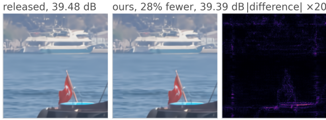
Figure 53. What the saving looks like. The same bitstream decoded by the released decoder and by ours at the 0.1 dB operating point. The crop is the tile that gave up the most quality on this frame, chosen automatically rather than by eye, so it shows the method's worst case here and not a flattering one.
