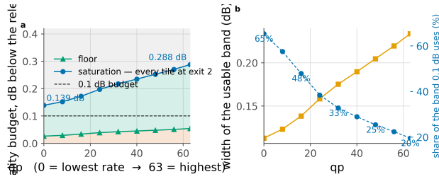
Figure 54. Three regions, and only the middle one is a design choice. Below the floor no allocation meets the budget; above saturation every tile already takes the cheapest exit and a looser budget buys nothing. The 0.1 dB budget uses 65% of the band at the lowest rate and 20% at the highest, which is why the same budget behaves so differently at the two ends of the rate range.
