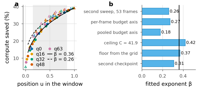
Figure 15. The collapse, and what the exponent is sensitive to. a The rescaled points from two sweeps of the pinned checkpoint, filled circles for the 106-frame grid and open triangles for the 53-frame frontier, with the power law fitted to each over the shaded window. The two sweeps of one checkpoint do not lie on one curve. b The exponent under one change at a time, with the vertical line at the exponent of the first row of Table 49. The change of checkpoint, which the main paper reads as a finding, is the smallest of the six.
