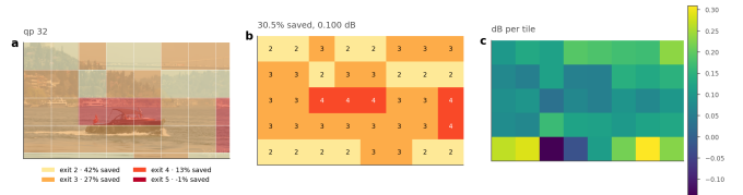
Figure 15. Where the decoder spends. Bosphorus at q32, a 0.1 dB budget. (a) the assignment overlaid on the frame, (b) the exit index per tile, (c) the quality each tile gives up, against its own full-depth reference. Water and sky leave at the shallowest exit; the boat and the shoreline run deep.
