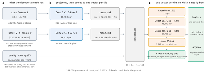
Figure 8. The router head. a , the three things it reads, all already held by the decoder. b , each projected by a 1 \times 1 , then reduced to one vector per tile by its mean and standard deviation. c , a three-layer perceptron, one pass per tile. Every shape and parameter count is read off the module when the figure is drawn.
