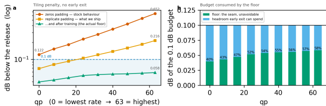
Figure 11. The tiling penalty across the whole rate range , every tile at full depth. The two steps that matter cost nothing, and the largest single factor is training the ladder with the seam present. Panel (b): the floor is charged inside the distortion budget and consumes a growing share of it.
