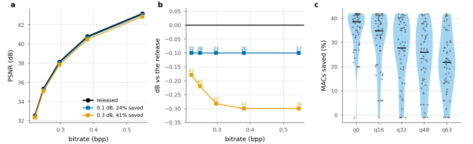
Figure 14. The plane a codec is read on, and the spread behind the mean. a , operating points against the released curve. b , the same with the quality axis expanded; labels are compute saved. c , per sequence at a matched point near 0.1 dB; one dot per sequence, bar is the median.
