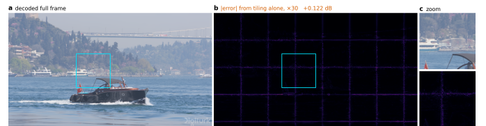
Figure 9. The artefact, before anything is done about it. Bosphorus at 1080p, quality index 63, zero padding at the tile border. a , the frame decoded in one piece. b , the same bitstream and weights decoded in 256 pixel tiles, every tile at full depth: the difference between the two, amplified 30 times. c , the boxed region of each.
