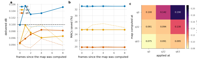
Figure 24. Reusing an exit map. Solid is the transferred map, dashed the one recomputed in place. a, b: reuse across frames of the same sequence. c: reuse across quality index; the entry is the delivered distortion against a 0.1 dB budget.
