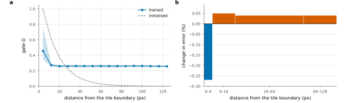
Figure 12. A learned deblocking filter , gated by position within a tile and applied once to the stitched frame, for 0.95% of the decode. a , the trained gate against distance from the boundary, beside its initialisation. b , the change in error by that distance; bar width is the share of pixels, so bar area is the contribution to the frame. It wins on the 6.2% of pixels nearest a boundary and loses on the 94% beyond.
