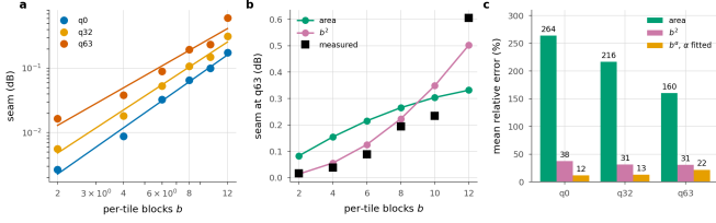
Figure 10. The seam against per-tile depth. a , the measurement with the fitted power law. b , both models against q63, one free scale each. c , mean relative error. The area fraction saturates once the border reaches every pixel; the penalty does not.
