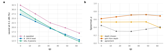
Figure 22. The calibrated bit rule. a Saving at 0.1 dB; shaded where the calibrated bit rule beats the trained head. b What a tile's bit count is correlated with, against how often the rule agrees with the oracle outright; dotted is the head's own held-out agreement.
