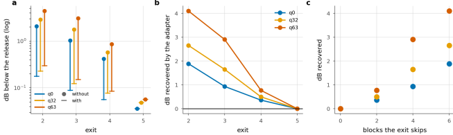
Figure 7. What the adapters are worth. a , each exit with and without its adapter. b , the dB the adapter recovers. c , the same against the number of blocks the exit skips, which is the design rationale measured.
