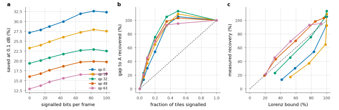
Figure 23. Partial signalling. a, saving against the bits spent on the map; each line runs from B on the left to A on the right. b, the same normalised by the A-to-B gap; dashed is proportional recovery. c, against the fixed- \lambda Lorenz bound; points above the dashed line are allocations one multiplier cannot reach.
