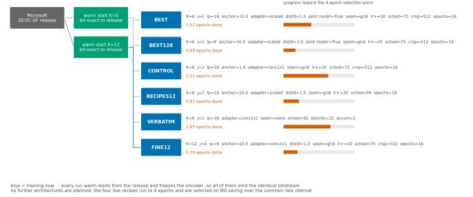
Figure 3. Lineage of the training runs. Every run warm-starts from the released decoder through one of two remaps, one per ladder size, and freezes the encoder, so all of them consume the identical bitstream. The flags shown are the ones that differ between runs. The progress bars are a snapshot taken on 2026-08-18 and the runs have advanced since; the current position of the run this paper reports is given in A.10.
