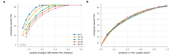
Figure 19. The band is the rate dependence. a Saving against the budget, with each rate's floor and saturation point ticked. b The same with the budget axis rescaled onto each rate's own band. Five curves become one; dashed is the one-parameter power law fitted to all of them.
