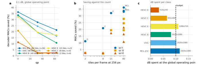
Figure 16. Saving by test class at one global operating point. \lambda is bisected once so the whole set lands on the budget, exactly as it would be in deployment; each class is then reported at that \lambda . The ordering follows tile count, not content.
