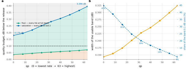
Figure 17. Three regions, and only the middle one is a design choice. Below the floor no allocation meets the budget; above saturation every tile already takes the cheapest exit. The 0.1 dB budget uses 45% of the band at the lowest rate and 9% at the highest.
