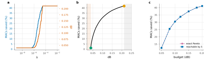
Figure 18. The structure of the allocation, on one frame. a , compute and distortion are monotone in the multiplier. b , the frontier between floor and saturation; shaded regions are infeasible or wasted. c , what the Lagrangian reaches against the exact Pareto set, enumerated by dynamic programming.
