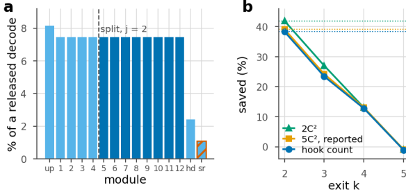
Figure 40. Where the arithmetic is, and what an exit saves. a , one released decode by module: the opening upsample, the twelve trunk blocks, the head, and the seam-repair pass this work adds (hatched). Light bars always run; dark bars are the eight blocks after the split that a tile can skip. b , the saving at each reachable exit under three prices for the same architecture, with each price’s ceiling dotted. Section B.5 is the table behind it.
