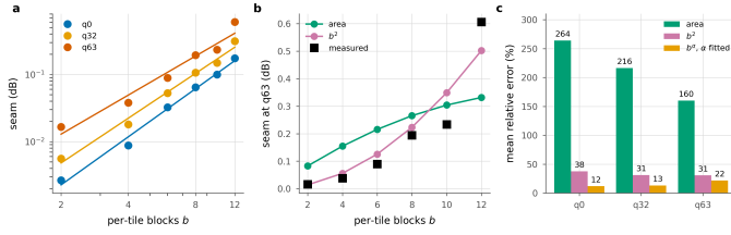
Figure 62. The seam against per-tile depth. a , the measurement with the fitted power law. b , both models against q63, one free scale each. c , mean relative error. The area fraction saturates once the border reaches every pixel and the penalty does not, which is where the area law fails as a predictor.
