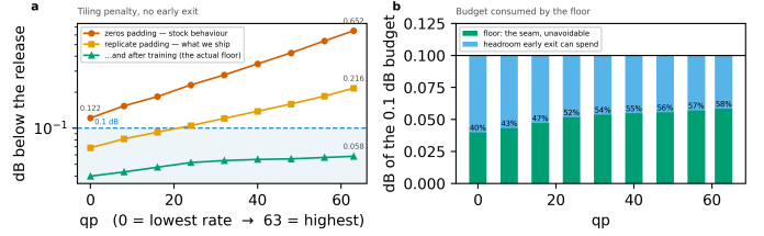
Figure 52. The tiling penalty across the whole rate range, every tile at full depth, so this is the floor and nothing else. a, the steps that reduce it, of which the two that matter cost no arithmetic; the largest single factor is training the ladder with the seam present. b, the floor as a share of the 0.1 dB budget: it is charged inside the budget and consumes a growing part of it as the rate rises, which is one of the two reasons the saving falls with rate.
