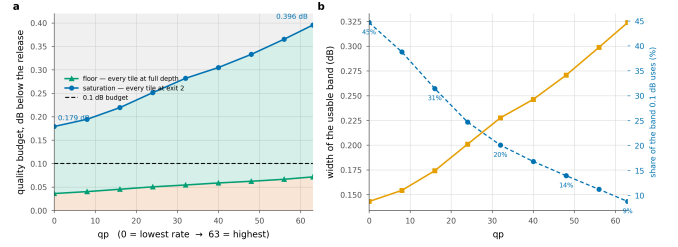
Figure 51. Three regions, and only the middle one is a design choice. Below the floor no allocation meets the budget; above saturation every tile already takes the cheapest exit and a looser budget buys nothing. The 0.1 dB budget uses 45% of the band at the lowest rate and 9% at the highest, which is why the same budget behaves so differently at the two ends of the rate range.
