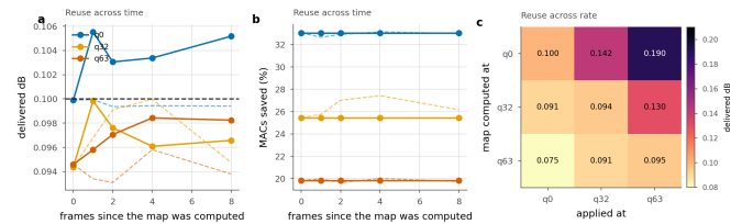
Figure 16. Reusing an exit map. Solid is the transferred map, dashed the one recomputed in place. a , b : reuse across frames of the same sequence. c : reuse across quality index; the entry is the delivered distortion against a 0.1 dB budget.
