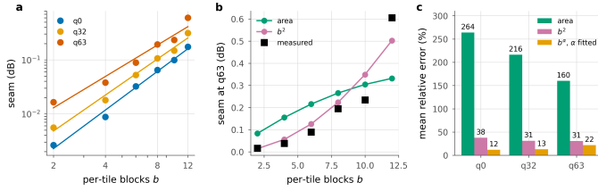
Figure 64. The seam against per-tile depth. a , the measurement with the fitted power law. b , both models against q63, one free scale each. c , mean relative error. The area fraction saturates once the border reaches every pixel and the penalty does not, which is where the area law fails as a predictor.
