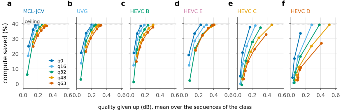
Figure 48. Compute saved against quality given up, one panel per class and one curve per quality index, from the seven budgets at which the frontier was measured. The dotted line is the architectural ceiling of 39.1%. Three things are visible that a table of operating points hides. The curves are steep and then flat, so most of the saving is bought in the first tenth of a decibel and the rest of the band buys little. The rate ordering is preserved at every budget, so a curve never crosses another within a panel. And the panels move to the right as resolution falls: MCL-JCV reaches the ceiling by 0.3 dB at every rate, while HEVC D needs 0.5 dB at q48 and does not reach it at q63 within the measured range.
