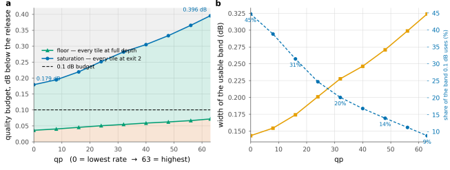
Figure 53. Three regions, and only the middle one is a design choice. Below the floor no allocation meets the budget; above saturation every tile already takes the cheapest exit and a looser budget buys nothing. The 0.1 dB budget uses 45% of the band at the lowest rate and 9% at the highest, which is why the same budget behaves so differently at the two ends of the rate range.
