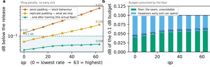
Figure 54. The tiling penalty across the whole rate range, every tile at full depth, so this is the floor and nothing else. a , the steps that reduce it, of which the two that matter cost no arithmetic; the largest single factor is training the ladder with the seam present. b , the floor as a share of the 0.1 dB budget: it is charged inside the budget and consumes a growing part of it as the rate rises, which is one of the two reasons the saving falls with rate.
