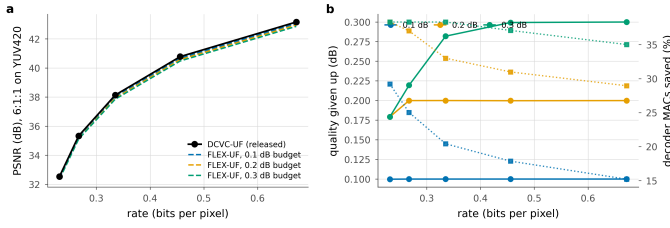
Figure 49. a , rate against quality over the five quality indices, the released DCVC-UF intra decoder and FLEX-UF at three budgets, on the 53 CTC intra frames. Both axes come from one pass over the same frames, and the encoders are asserted bit-identical on the weights before a shared rate is reported, because a shared x-axis is a claim rather than a convenience. b , the same difference magnified: the decibels each budget delivered, against the decoder arithmetic it bought on the right-hand axis.
