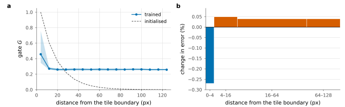
Figure 63. The learned deblocking filter, and where it wins. It is gated by position within a tile and applied once to the stitched frame, for 1.09% of the decode. a , the trained gate against distance from the boundary, beside its initialisation. b , the change in error by that distance; bar width is the share of pixels, so bar area is the contribution to the frame. It wins on the pixels nearest a boundary and loses on the rest, which is why a perfect gate still cannot pay for it.
