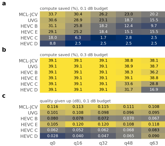
Figure 46. The same measurement as a grid, with the looser budget under it. a , compute saved at the 0.1 dB budget. b , the same at 0.3 dB, where every class at the three lowest rates has reached the architectural ceiling of 39.1% and only q48 and q63 are still making a choice. c , the quality actually given up at the 0.1 dB budget, which the set meets and no class does: at q0 the allocation spends 0.116 dB on MCL-JCV and 0.028 dB on HEVC D. The small classes are cheap in quality for the same reason they are poor in saving, that with two or eight tiles there is no fine-grained way to spend a budget. The 0.5 dB grid is not drawn because every one of its thirty cells is at the ceiling.
