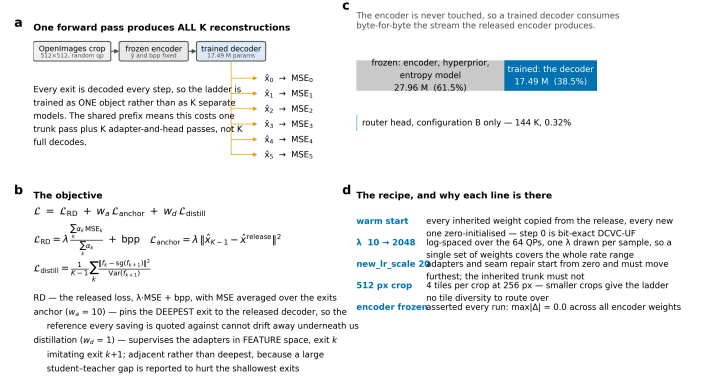
Figure 40. The training scheme. a, one forward pass produces all K reconstructions, so the ladder is trained as one object. b, the three loss terms. c, the encoder is never touched. d, why each line of the recipe is there. The figure is a schematic drawn from the model definition; the parameter counts it carries are the ones tabulated in A.5.
