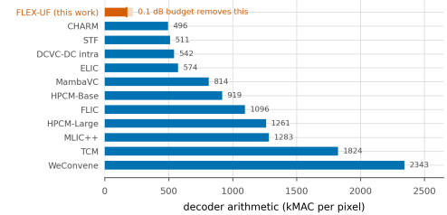
Figure 2. Every published decoder is one number. Arithmetic per pixel for the eleven image codecs of Table 2, and for the intra decoder this work modifies. Costs are comparable here even though the BD-Rate anchors are not, which is why this axis and not a rate-distortion one. The bar at the top is the same decoder as the rest of the paper: a 0.1 dB budget removes the pale section, and how much it removes depends on the picture.
