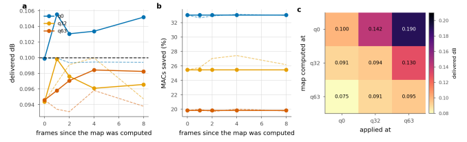
Figure 28. Reusing an exit map. Solid is the transferred map, dashed the one recomputed in place. a , b : reuse across frames of the same sequence. c : reuse across quality index; the entry is the delivered distortion against a 0.1 dB budget.
