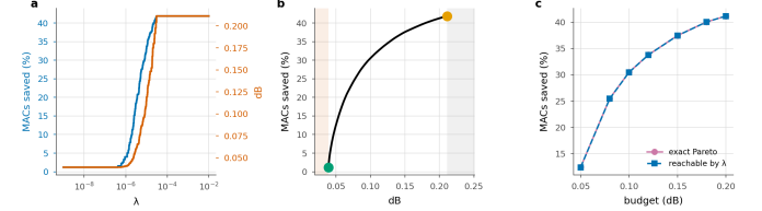
Figure 19. The structure of the allocation , on one frame. a , compute and distortion are monotone in the multiplier. b , the frontier between floor and saturation; shaded regions are infeasible or wasted. c , what the Lagrangian reaches against the exact Pareto set, enumerated by dynamic programming.
