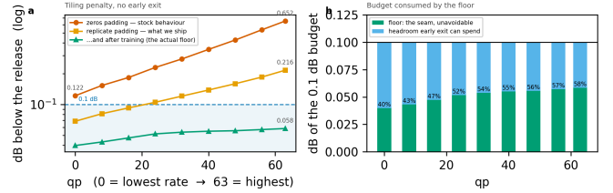
Figure 13. The tiling penalty across the whole rate range , every tile at full depth. The two steps that matter cost nothing, and the largest single factor is training the ladder with the seam present. Panel (b): the floor is charged inside the distortion budget and consumes a growing share of it.
