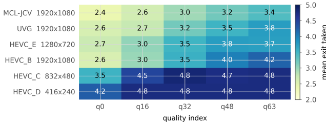
Figure 19. How deep each class has to go. Mean exit taken by the tiles of each test class at the 0.1 dB budget, ordered by that mean. Resolution is the strongest predictor: the 416x240 class has two tiles a frame and almost no choice, and the 1080p classes have forty and use the whole ladder. This is the dependence Section 5.3 measures, seen per class rather than pooled.
