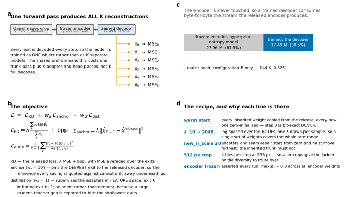
Figure 46. The training scheme. a, one forward pass produces all K reconstructions, so the ladder is trained as one object. b, the three loss terms. c, the encoder is never touched. d, why each line of the recipe is there. The figure is a schematic drawn from the model definition; the parameter counts it carries are the ones tabulated in A.5.
