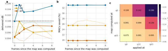
Figure 25. Reusing an exit map. Solid is the transferred map, dashed the one recomputed in place. a, b: reuse across frames of the same sequence. c: reuse across quality index; the entry is the delivered distortion against a 0.1 dB budget.
