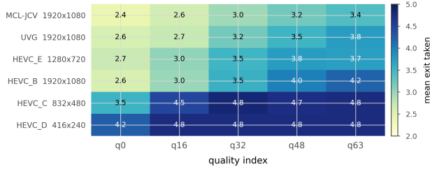
Figure 21. How deep each class has to go. Mean exit taken by the tiles of each test class at the 0.1 dB budget, ordered by that mean. Resolution is the strongest predictor: the 416×240 class has two tiles a frame and almost no choice, and the 1080p classes have forty and use the whole ladder. This is the dependence Section 5.3 measures, seen per class rather than pooled.
