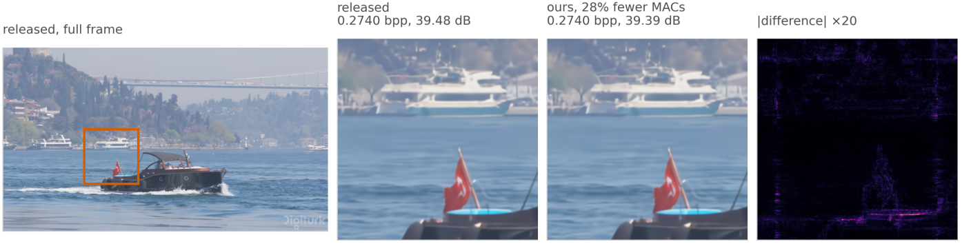
Figure 30. What 28.1% of the arithmetic costs, to look at. Bosphorus at q32, one frame, with \lambda bisected on that frame to 0.100 dB. Both crops are decoded from the same latent at 0.2740 bpp: the released decoder reaches 39.48 dB and the routed decode 39.39 dB. The crop is centred on the tile that gave up the most, tile 18 of 40, not on a flattering one. Right, the absolute difference at \times 20 .
