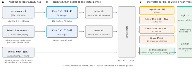
Figure 9. The router head. a , the three things it reads, all already held by the decoder. b , each projected by a 1 \times 1 , then reduced to one vector per tile by its mean and standard deviation. c , a three-layer perceptron, one pass per tile. Every shape and parameter count is read off the module when the figure is drawn.
