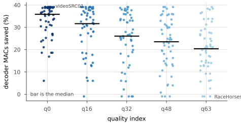
Figure 19. What the set mean hides. Every test sequence as a point, at the 0.1 dB budget; the bar is the median. At the lowest rate the saving runs from 6.0% to 39.1% across the 53 sequences and at the highest from -1.0% to 39.1%. The spread within a rate is larger than the difference between rates, and it is content, not noise: the same sequences sit at the same end of it at every rate.
