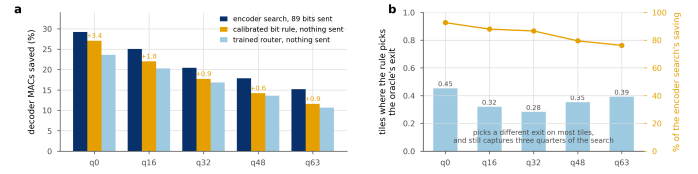
Figure 29. Three ways to choose an exit. a, saving at the 0.1 dB budget. The encoder search sees the source and sends 89 bits a frame; the other two send nothing. The bit rule beats the trained head at every rate, by the margin printed above it, with no learned parameters against the head's 144,030. b, bars are the tiles on which the rule picks the exit the search would have, and the line is the fraction of the search's saving it nonetheless captures. Picking a different exit on most tiles costs it far less than picking a different exit sounds like it should, which is the case against training a router on exit labels.
