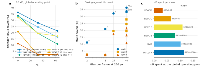
Figure 20. Saving by test class at one global operating point. \lambda is bisected once so the whole set lands on the budget, exactly as it would be in deployment; each class is then reported at that \lambda . The ordering follows tile count, not content.
