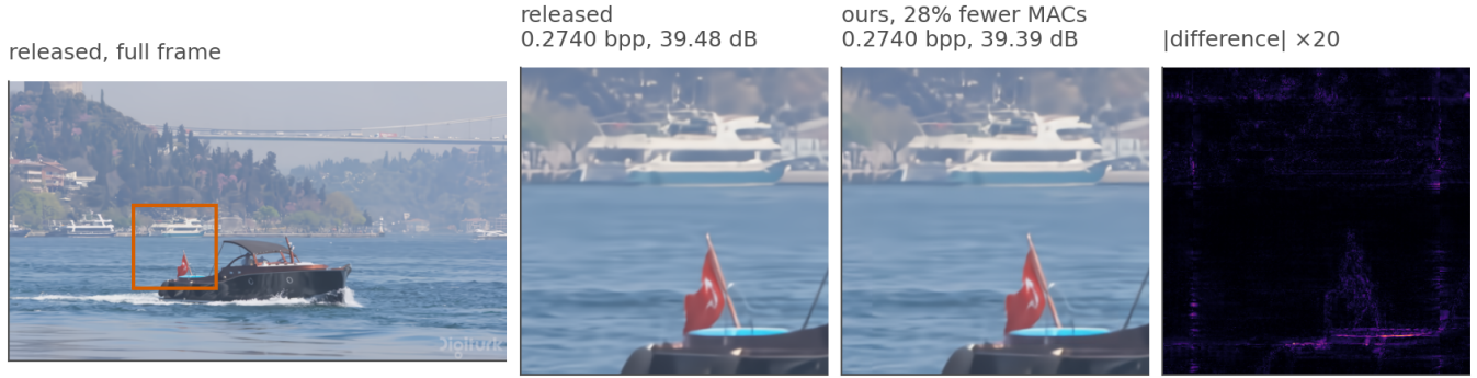
Figure 34. What 28.1% of the arithmetic costs, to look at. Bosphorus at q32, one frame, with \lambda bisected on that frame to 0.100 dB. Both crops are decoded from the same latent at 0.2740 bpp: the released decoder reaches 39.48 dB and the routed decode 39.39 dB. The crop is centred on the tile that gave up the most, tile 18 of 40, not on a flattering one. Right, the absolute difference at \times 20 .
