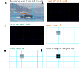
Figure 15. What the deblocking pass does to a picture. Bosphorus at q63, the rate where the seam is worst, decoded twice from one latent with every tile at full depth. a , the frame and its 5 \times 8 grid. b , c , the error against a full-frame decode of the same latent, amplified 25 times, with the pass off and on. d , e , one grid crossing in the picture itself. f , what the pass changed there. It recovers 0.005 dB of the 0.041 dB that tiling costs on this frame, which is the measurement behind the section title.
