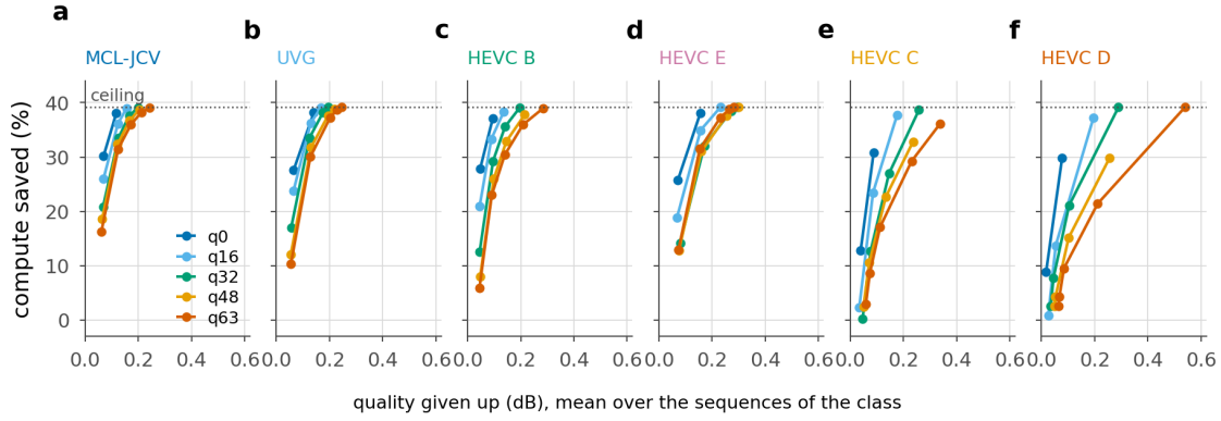
Figure 46. Compute saved against quality given up, one panel per class and one curve per quality index, from the seven budgets at which the frontier was measured. The dotted line is the architectural ceiling of 39.1%. Three things are visible that a table of operating points hides. The curves are steep and then flat, so most of the saving is bought in the first tenth of a decibel and the rest of the band buys little. The rate ordering is preserved at every budget, so a curve never crosses another within a panel. And the panels move to the right as resolution falls: MCL-JCV reaches the ceiling by 0.3 dB at every rate, while HEVC D needs 0.5 dB at q48 and does not reach it at q63 within the measured range.
