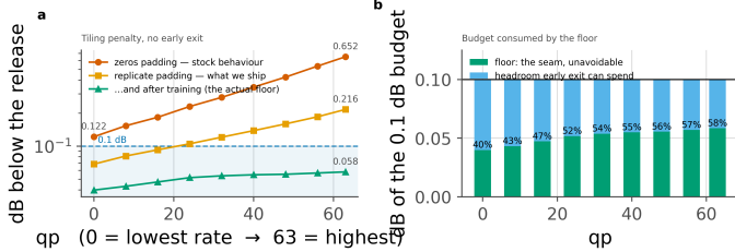
Figure 53. The tiling penalty across the whole rate range, every tile at full depth, so this is the floor and nothing else. a , the steps that reduce it, of which the two that matter cost no arithmetic; the largest single factor is training the ladder with the seam present. b , the floor as a share of the 0.1 dB budget: it is charged inside the budget and consumes a growing part of it as the rate rises, which is one of the two reasons the saving falls with rate.
