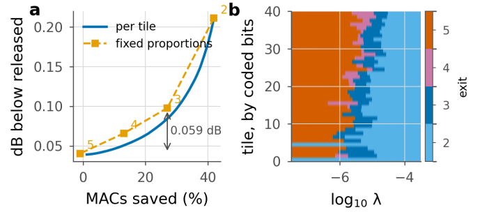
Figure 43. The two achievable sets, on one frame. a , the per-tile frontier of Theorem 4 traced by sweeping \lambda , against the fixed-proportion chain of Proposition 3 through the four uniform-depth points, labelled by exit. The per-tile curve lies below the chain everywhere between the vertices, by 0.059 dB at the exit-3 vertex. b , the exit each of the 40 tiles takes as \lambda rises, tiles ordered by the bits the entropy coder spent on them. Every row is non-increasing, which is Proposition 2 per tile, and the rows differ, which is what Theorem 4 buys over Proposition 3. The bottom row is a tile that never leaves the shallowest exit.
