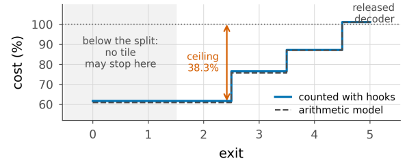
Figure 40. The ladder, priced. What a tile costs at each exit, as a percentage of one released decode, counted with hooks on the executed pass and beside the arithmetic model the argmin uses. Exits below the split depth are not distinct, because the first j groups run for every tile whatever it does. The deepest exit costs slightly more than the release, which is the full-frame deblocking pass. Reported savings in the paper are the hook count.
