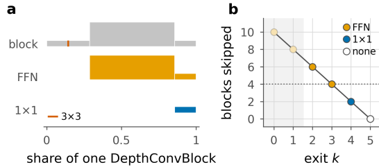
Figure 37. Inside an exit adapter. a , one DepthConvBlock and the two adapters, drawn to scale: bar length is a share of the block, bar height the channel width written. Neither adapter contains the block's only 3×3 (the hairline rule), so neither adds receptive field or seam penalty, which is the design constraint the seam measurement imposes. b , blocks skipped per exit, coloured by adapter; the rule switches to the FFN at four skipped blocks. Lengths are counted with hooks off the modules themselves.
