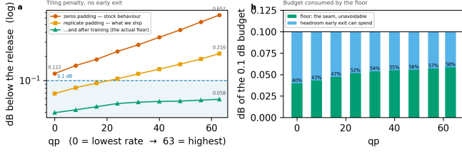
Figure 5. The tiling penalty across the whole rate range , every tile at full depth. The two steps that matter cost nothing, and the largest single factor is training the ladder with the seam present. Right: the floor is charged inside the quality budget and consumes a growing share of it.
