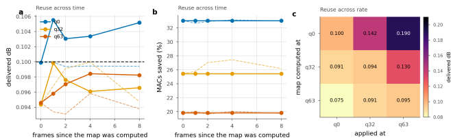
Figure 13. Reusing an exit map. Solid is the transferred map, dashed the one recomputed in place. a, b: reuse across frames of the same sequence. c: reuse across quality index; the entry is the delivered distortion against a 0.1 dB budget.
