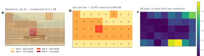
Figure 9. Where the decoder spends. (a) the assignment overlaid on the frame, (b) the exit index per tile, (c) the quality each tile gives up against its own full-depth reference. Water and sky leave at the shallowest rung; the boat and shoreline run deep.
