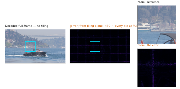
Figure 3. The artefact, before anything is done about it. One frame decoded twice from the same bitstream with the same weights, every tile at full depth — no early exit anywhere. The only difference is that the right-hand decode was tiled. The error map is the tile lattice and nothing else.
