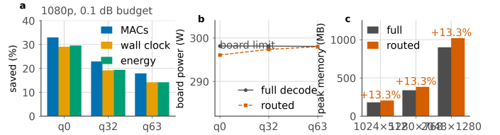
Figure 33. Three units for one saving. a, the same routed decode measured as arithmetic, as wall clock and as joules per frame, at 1080p and a 0.1 dB budget. Energy follows the clock, not the arithmetic. b, why: the board draws the same power either way, because the later groups run on a shrinking set of tiles and a partly idle GPU still draws its static power. c, peak memory, which routing raises rather than lowers, by 13.3% at every resolution that fitted on the card.
