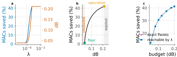
Figure 23. The structure of the allocation, on one frame. a, compute and distortion are monotone in the multiplier. b, the frontier, with both ends and both dead bands marked on the panel. c, what the Lagrangian reaches against the exact Pareto set, enumerated by dynamic programming.
