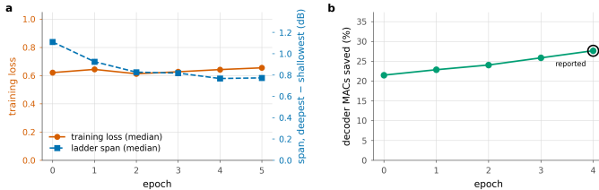
Figure 34. The run had not converged. Measured saving at the 0.1 dB budget on the 53 test frames, hook-counted, one point per completed epoch of the reported run. The circled point is the checkpoint this paper reports. The training loss over the same epochs is flat; the supplement shows the two together.
