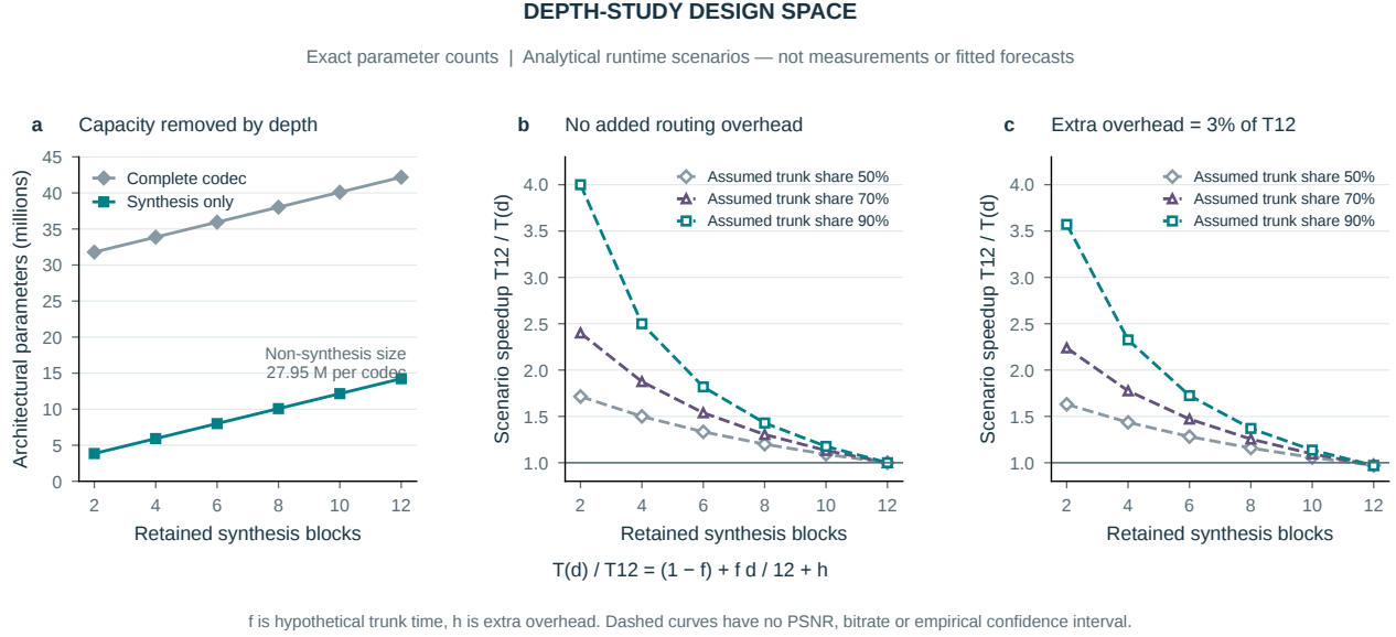
Figure S8. A transparent design-space illustration for unfinished experiments. a , Exact architectural parameter counts. b,c , Analytical runtime sensitivity to assumed trunk-time share and added overhead. Open markers and dashed lines denote assumptions, not measurements or fitted forecasts. No quality or bitrate outcome is assigned to an unfinished model.
