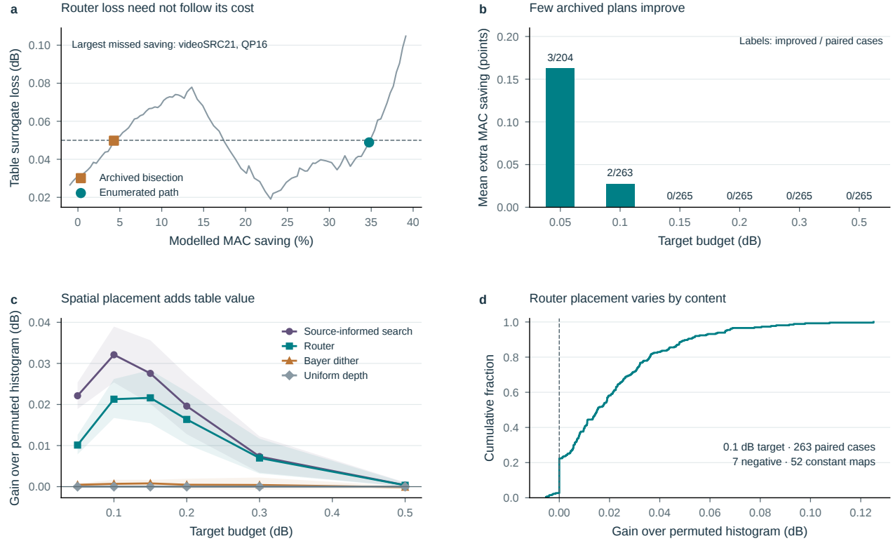
Figure S5. Control-path and assignment diagnostics. a , The explicitly selected largest missed router saving illustrates non-monotone table loss. b , Mean paired improvement from enumerating the router path; labels show improved and paired counts. Newly feasible cases are excluded from these means. c , Exact expected-shuffle comparison at unchanged exit histograms, with 95% sequence-cluster intervals. d , Router placement-gain distribution at 0.1 dB. All results are CPU analyses of padded error tables; none measures new final-image quality or latency.
