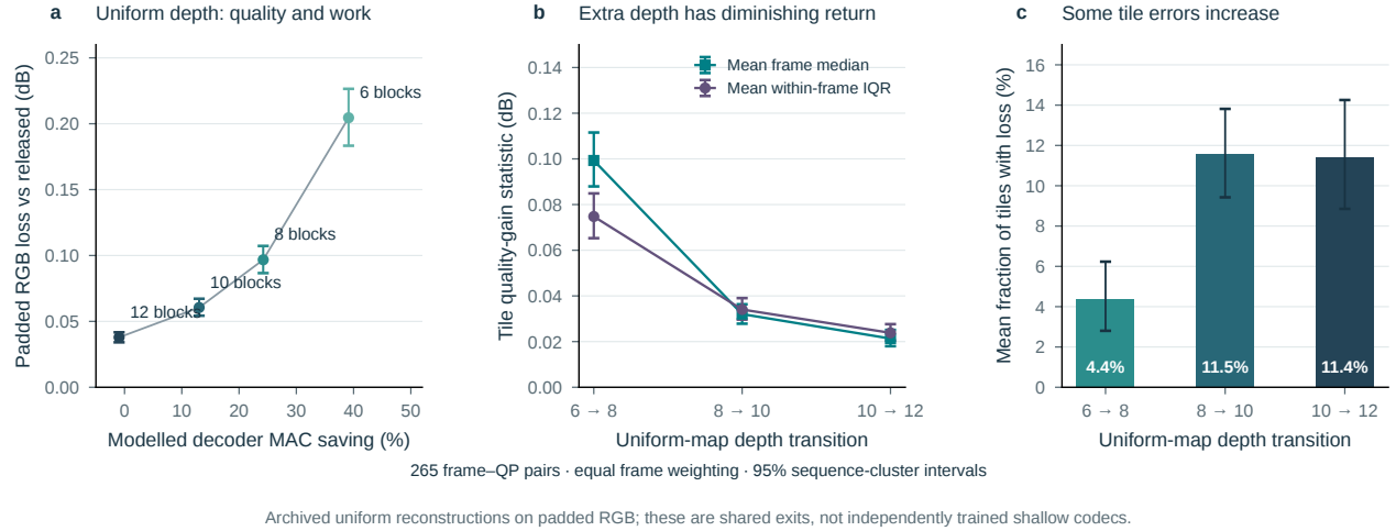
Figure S4. The value of additional depth varies across regions. a , Uniform-depth padded RGB quality against the released anchor and the recorded MAC model. b , Mean frame-median tile improvement and mean within-frame IQR for adjacent depths. c , Mean fraction of tiles whose error increases. Error bars are 95% sequence-cluster intervals. These are actual archived uniform reconstructions; neighbouring depths change together, and independent shallow codecs are not represented.
